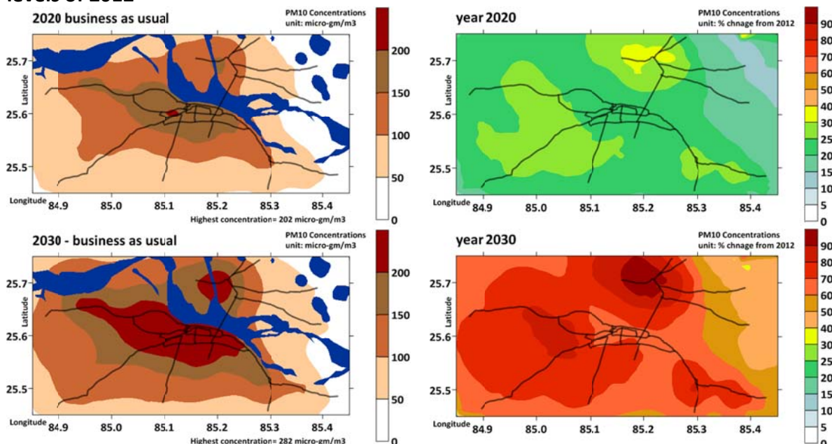
Figure 21: (a) Modeled annual average PM 10 concentrations under the business as usual scenario for 2020 and 2030; (b) Percentage increase in the concentrations compared to levels of 2012
