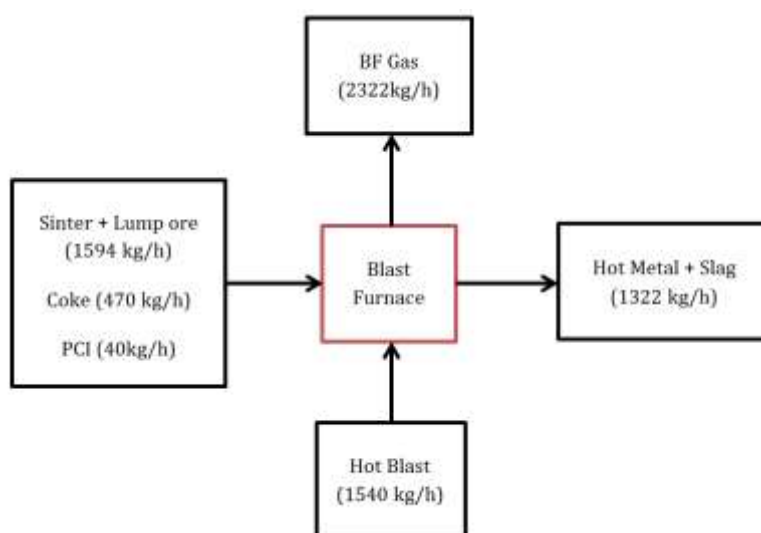
Figure 14: Material Balance of Blast Furnace with Coke and PCI Input
