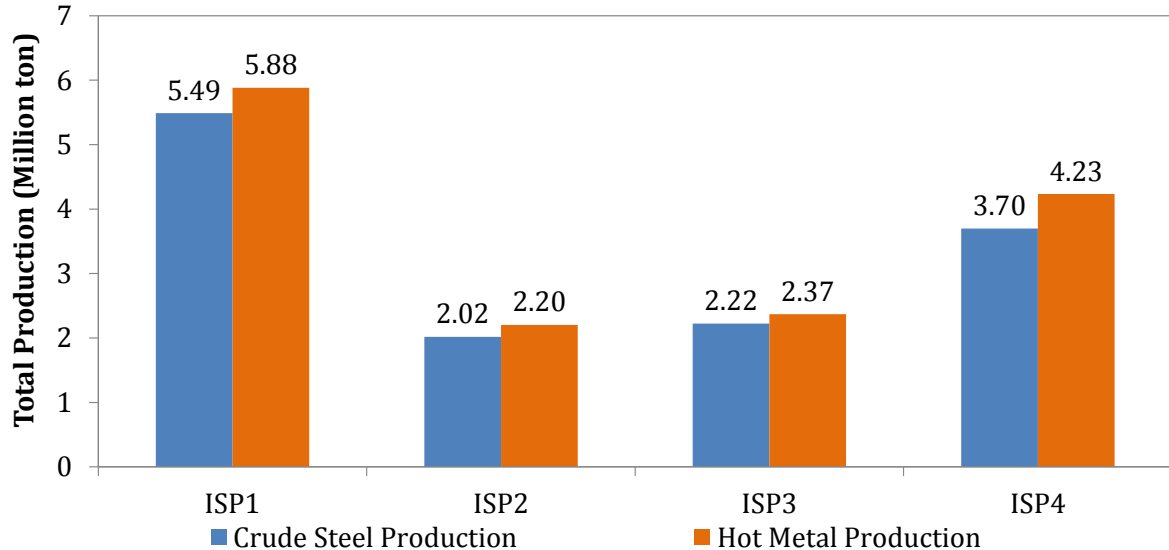
Figure 64: Crude Steel and Hot Metal Production Comparison for Sample ISP Plants
