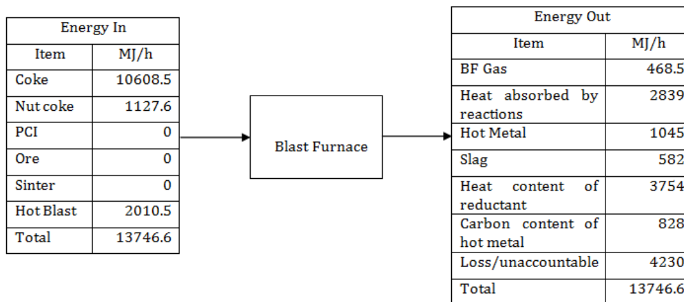
Figure 13: Energy Balance of Blast Furnace with Coke Input
