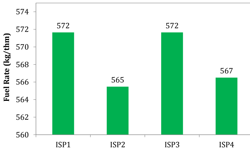
Figure 54: Blast Furnace Fuel Rate for Sample ISP Plants
