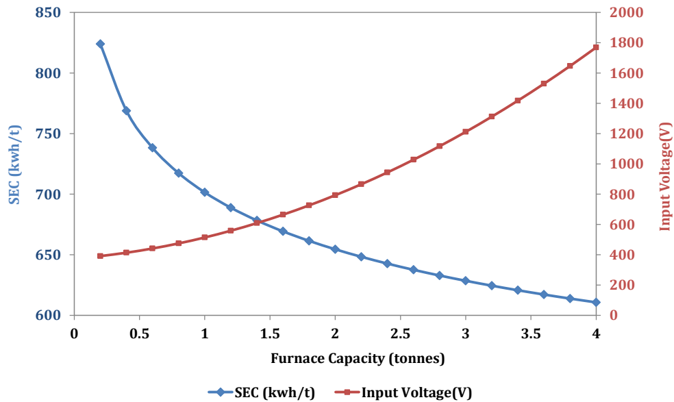
Figure 41: Energy consumption behaviour with increasing furnace capacity and input voltage
