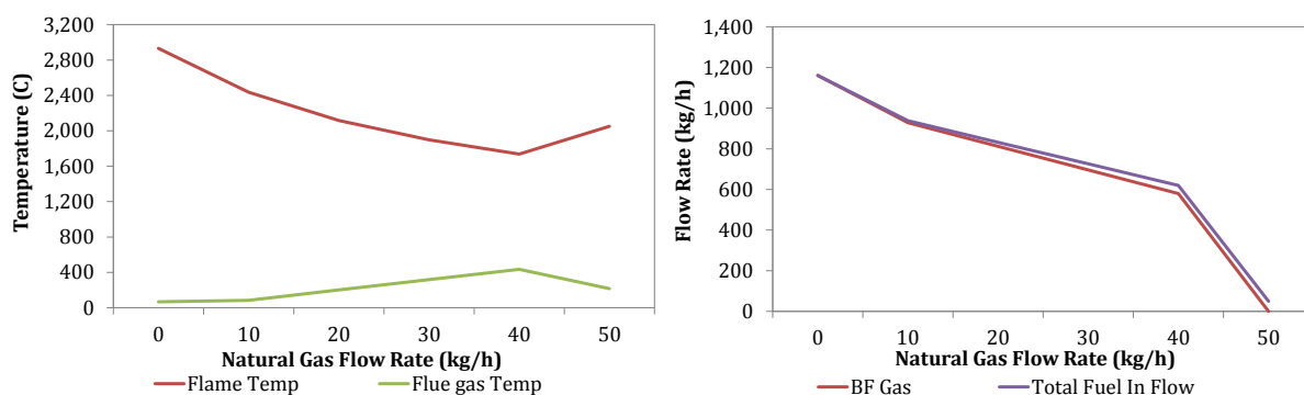
Figure 23: Hot Stove Performance with Mixed Fuel Injection
