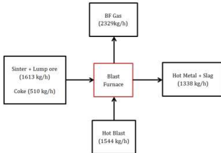
Figure 12: Material Balance of the BF with Coke Input
