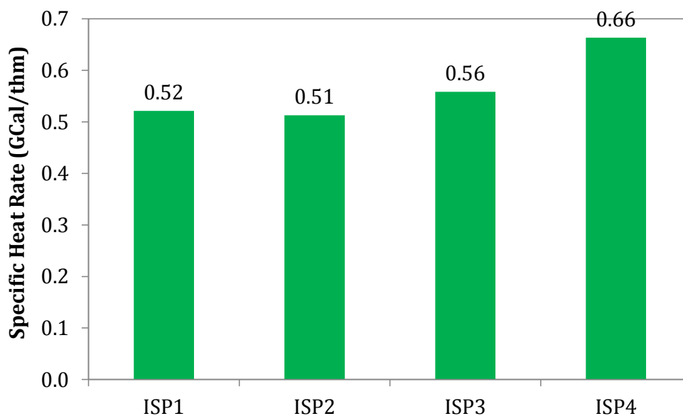
Figure 59: Specific Heat Rate in BF Hot Stove for Sample ISP Plants
