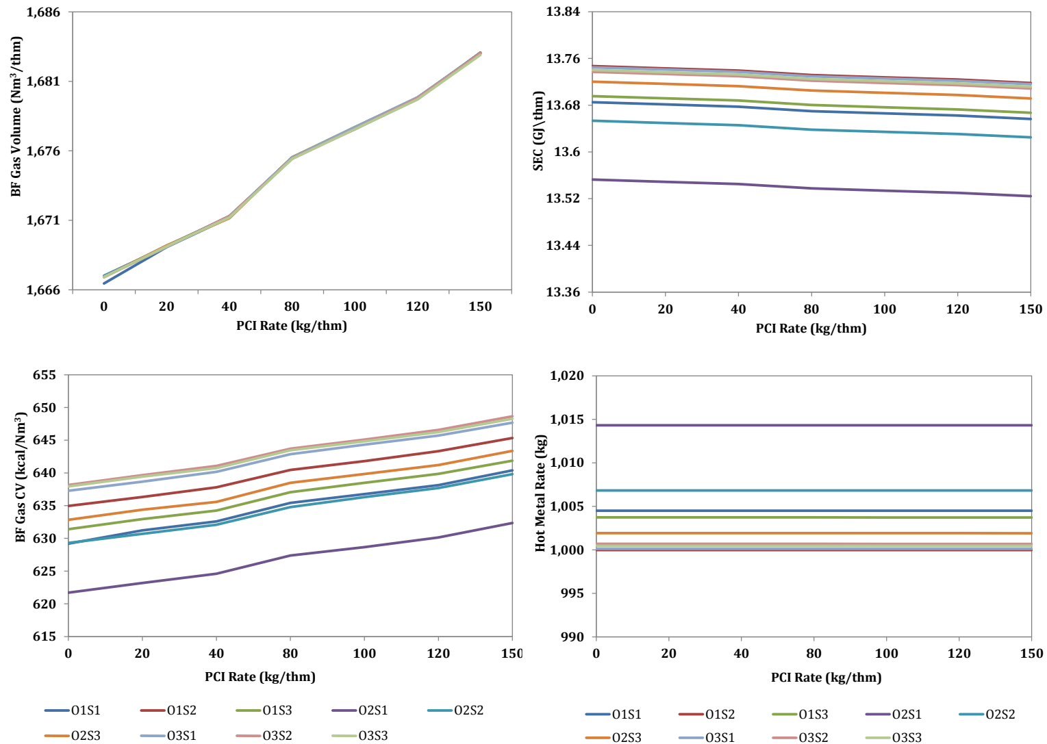
Figure 16: Gas Volume, SEC, BF Gas CV and Hot Metal Rate variation with PCI input rate
