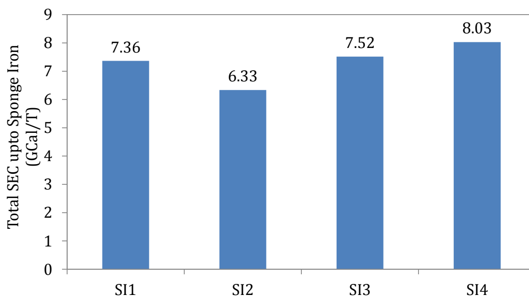
Figure 74: Total SEC up to sponge iron across sample SI plants
