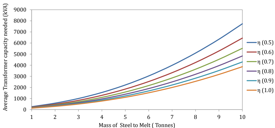
Figure 44: Sensitivity analysis for estimating the transformer capacity
