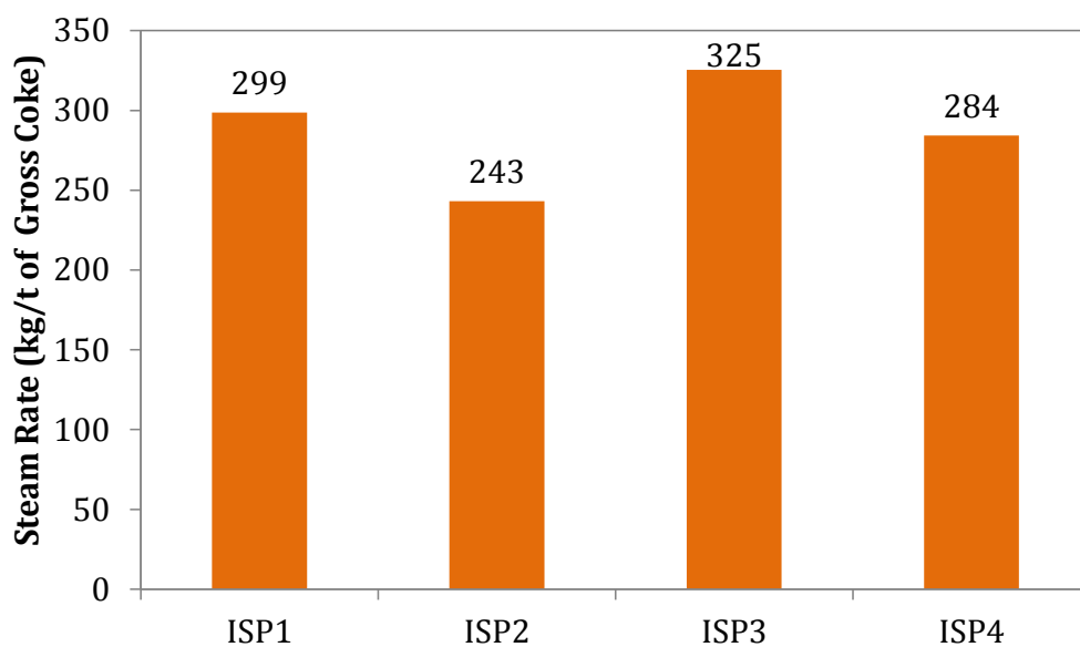
Figure 61: Steam Used in Coke Oven for Sample ISP Plants
