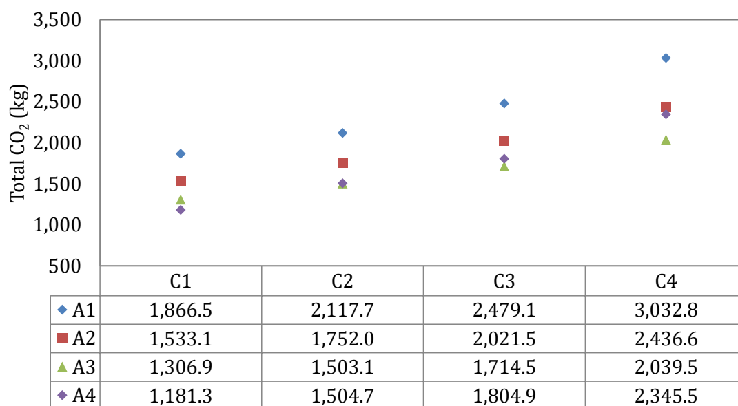
Figure 34: Total CO 2 emissions for different coals and for iron ore 2
