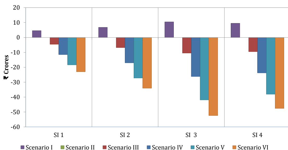
Figure 90: Savings beyond target under High Cost Scenario for sample Sponge Iron Plants
