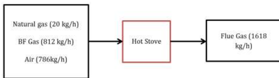
Figure 22: Material Balance across Hot Stove
