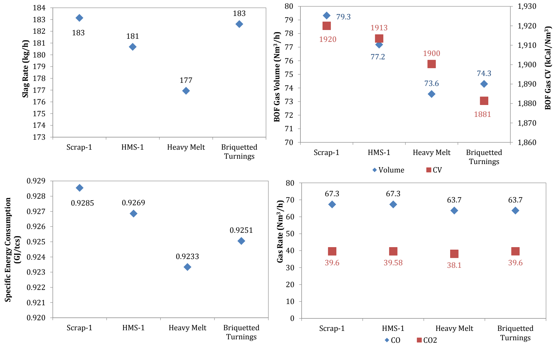
Figure 28: BOF Performance with Scrap Type
