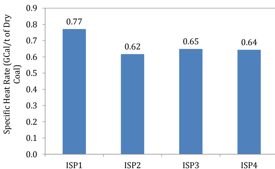
Figure 57: Specific Heat Consumption in Coke Oven for Sample ISP Plants
