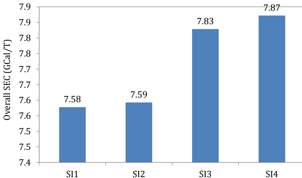
Figure 72: Specific Energy Consumption of different sample SI plants
