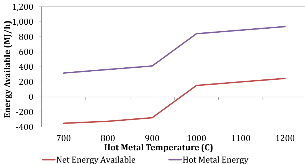
Figure 27: Hot Metal Energy Availability Variation with Temperature
