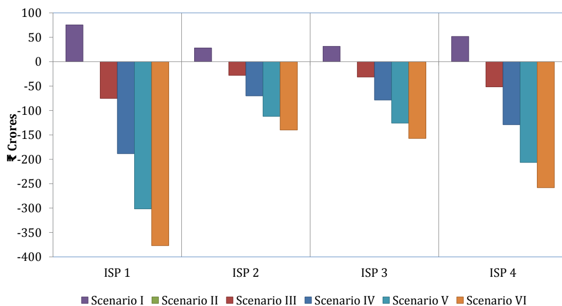
Figure 83: Savings beyond target under Low Cost Scenario for Sample ISP plants
