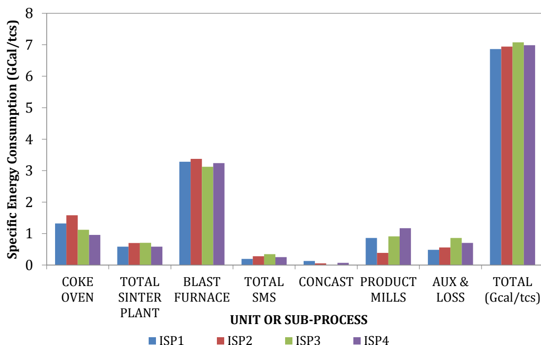
Figure 48: Energy Balance Comparison for Sample ISP Plants
