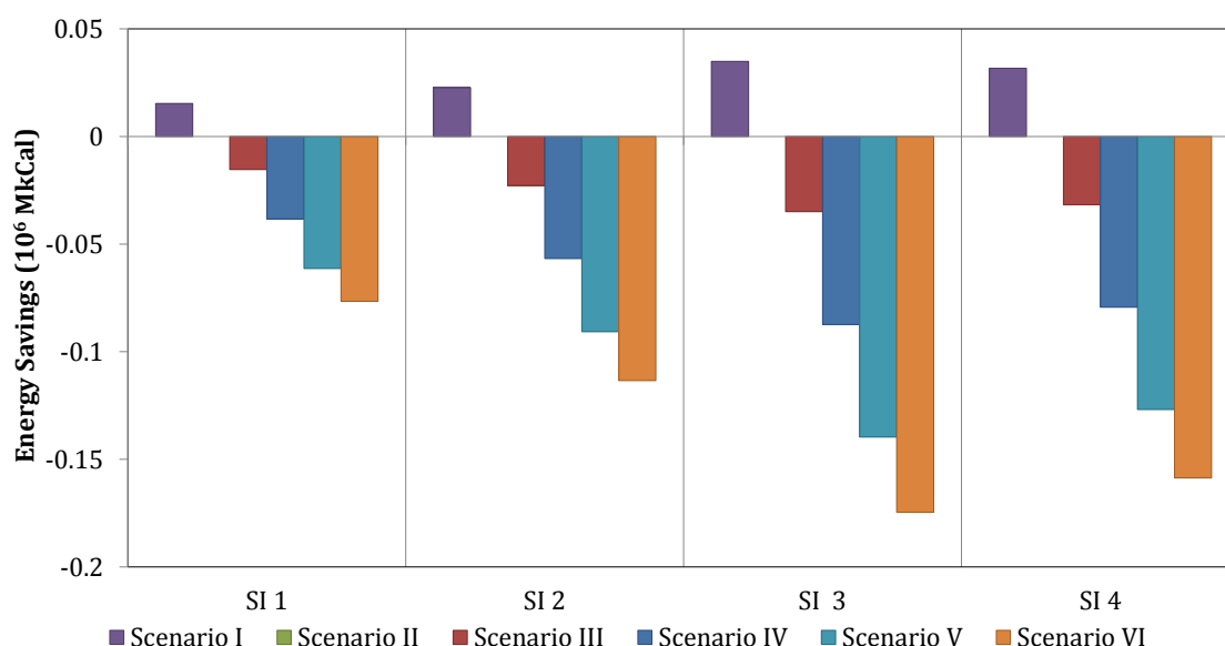
Figure 92: Energy saved beyond target for different Scenarios for sample sponge iron plants
