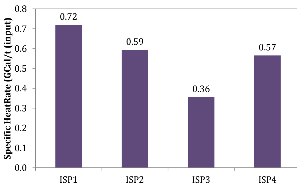
Figure 60: Specific Heat Consumption in Hot Mill for Sample ISP Plants
