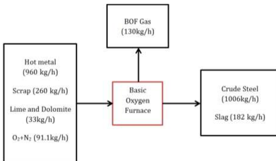
Figure 25: BOF Material Balance
