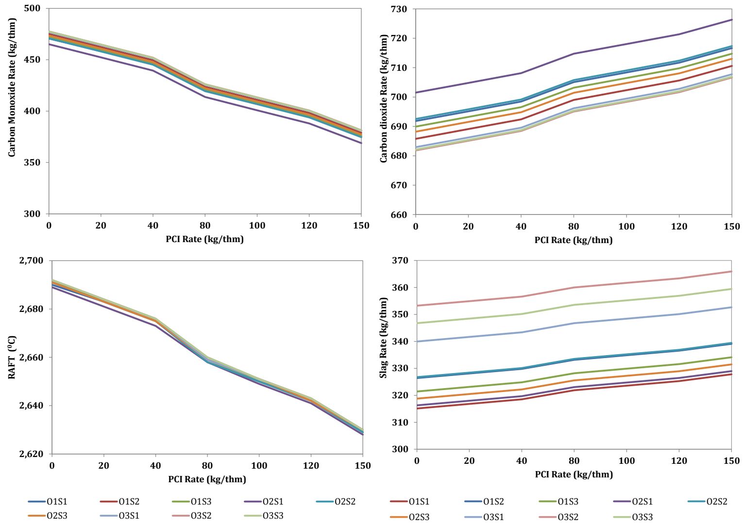
Figure 17: CO, CO 2 , RAFT and Slag Rate variation with PCI Rate
