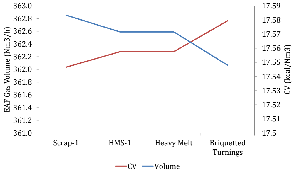
Figure 37: EAF gas volume and CV vs. scrap type
