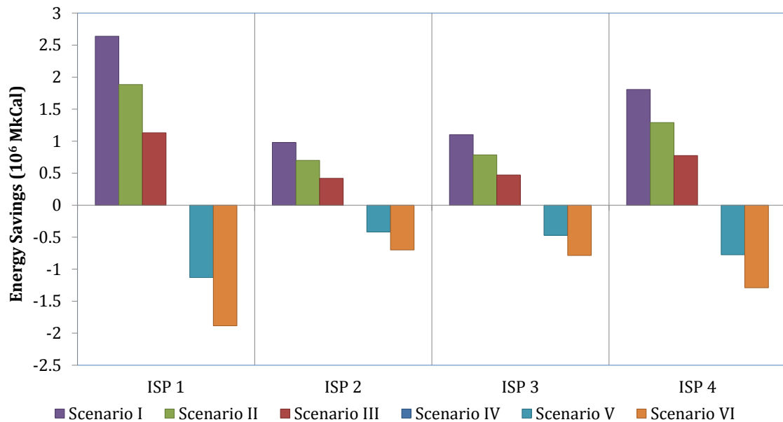
Figure 85: Energy saved at BL Production for different Scenarios for Sample ISP plants
