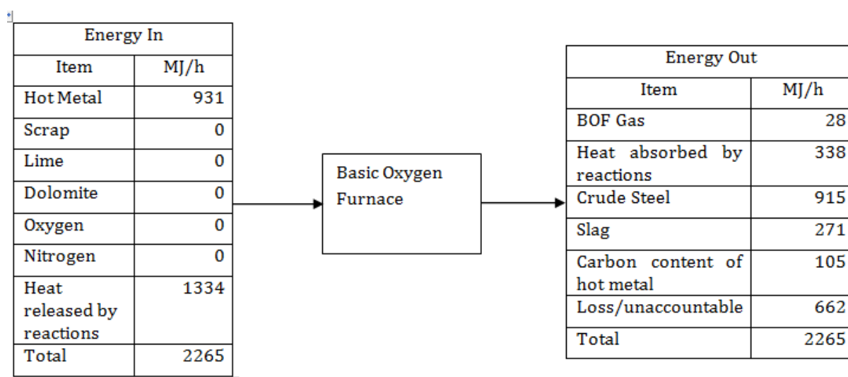
Figure 26: Energy Balance – BOF
