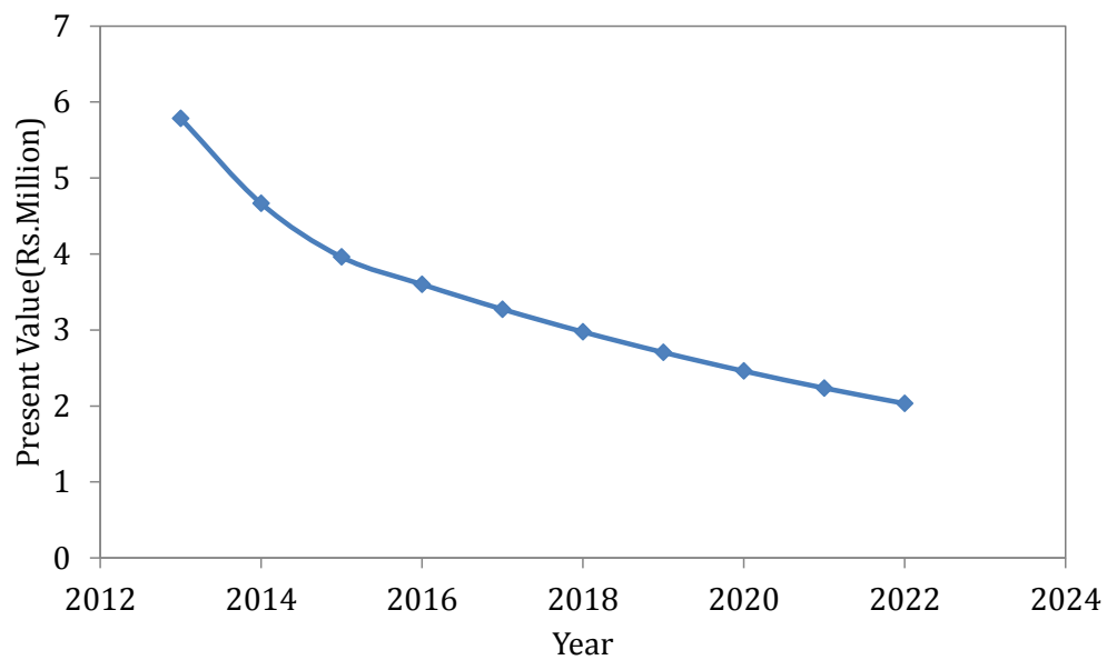
Figure 75: Present value of annual energy savings for variable speed drive
