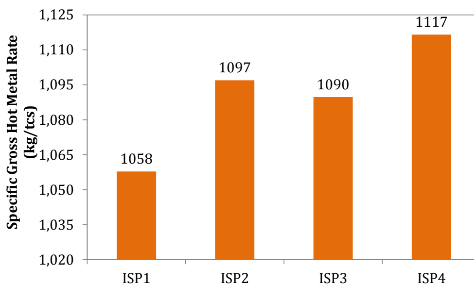
Figure 56: Specific Gross Hot Metal Consumption for Sample ISP Plants
