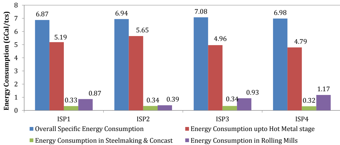
Figure 51: Specific Energy Consumption --- Comparison of Major Units for Sample ISP plants
