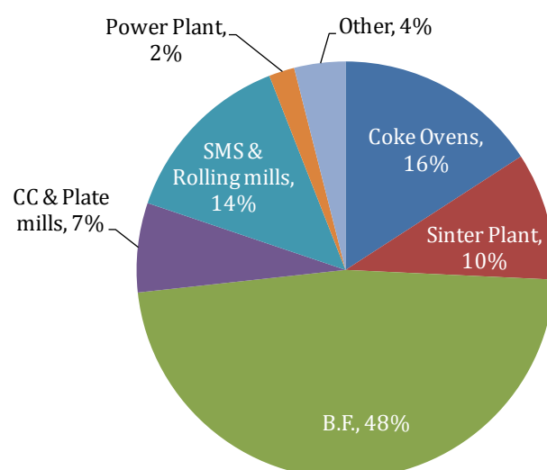
Figure 6: BF-BOF energy distribution in a typical integrated iron and steel plant (11)
