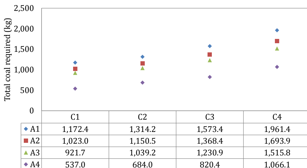
Figure 35: Coal required for different alternatives for iron ore 3
