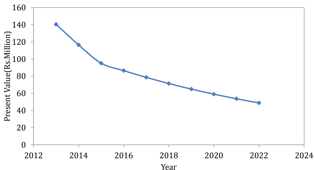
Figure 76: Present value of annual energy savings for Injection of coke oven gas in BF
