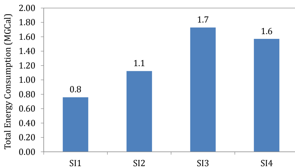
Figure 66: Thermal energy consumption across sample SI plants
