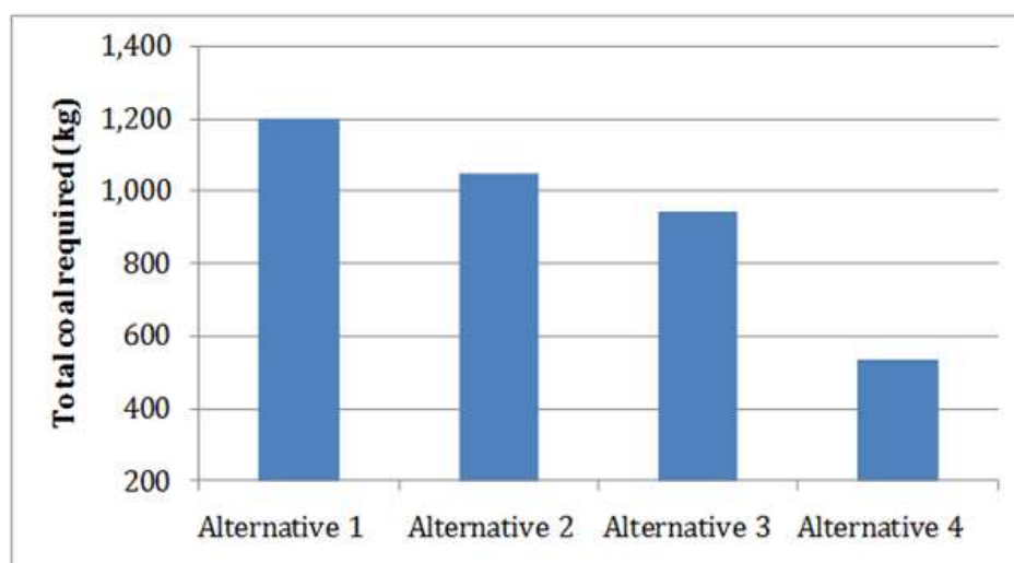
Figure 29: Total coal required for different alternatives
