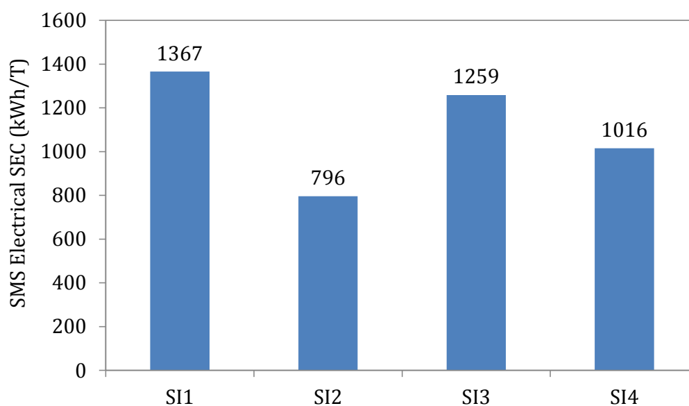
Figure 70: Electrical SEC of SMS across sample SI plants
