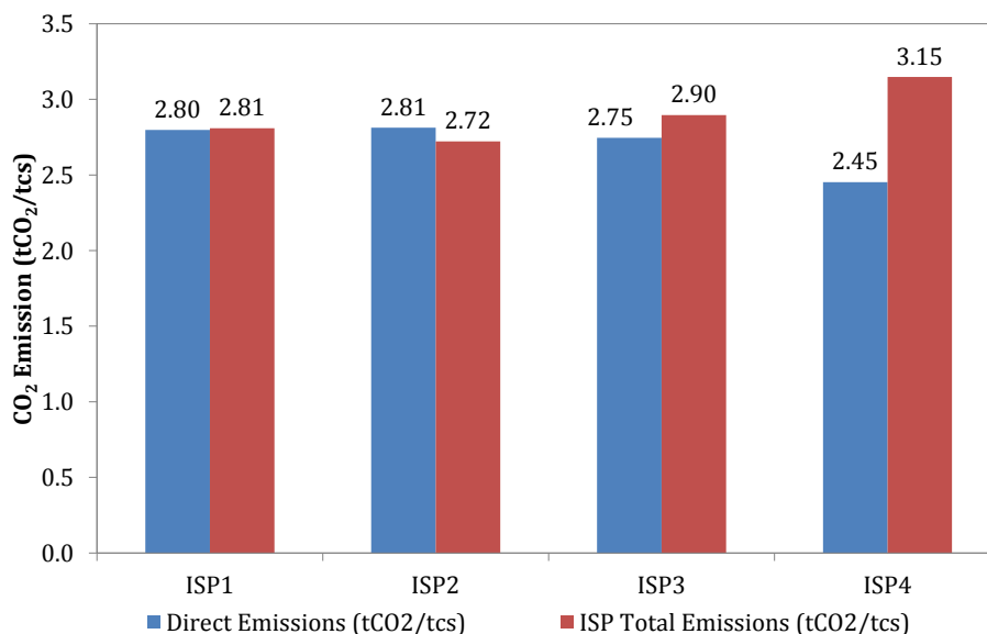
Figure 50: CO 2 Emission Comparison of Sample ISP Plants
