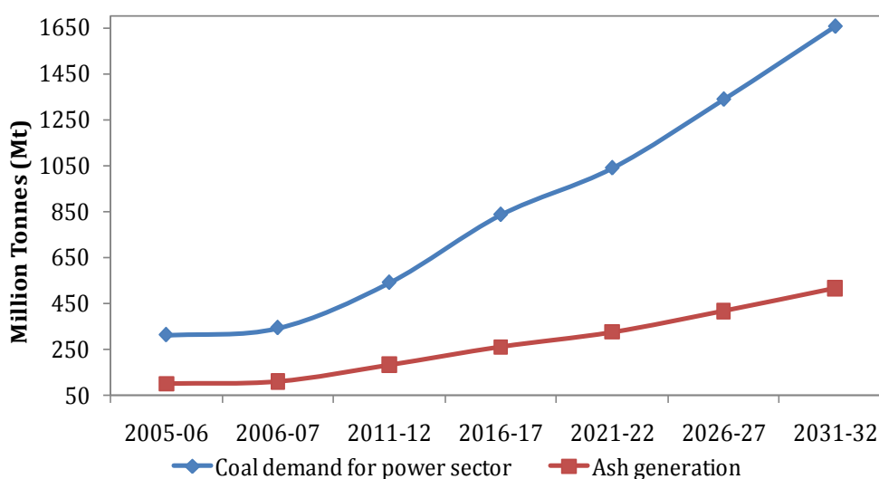
Figure 93: Projections for coal and ash generation (32)
