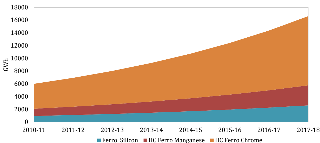
Figure 8: Projected energy consumption of Ferro Alloy in India
