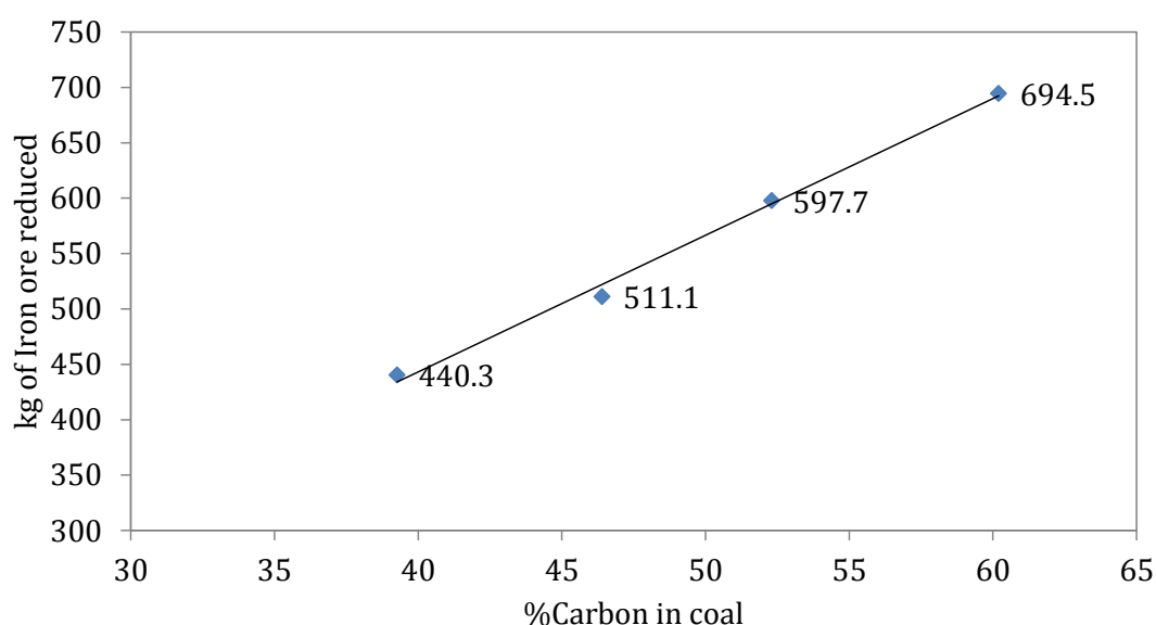
Figure 30: Iron ore reduced vs. %carbon in coal
