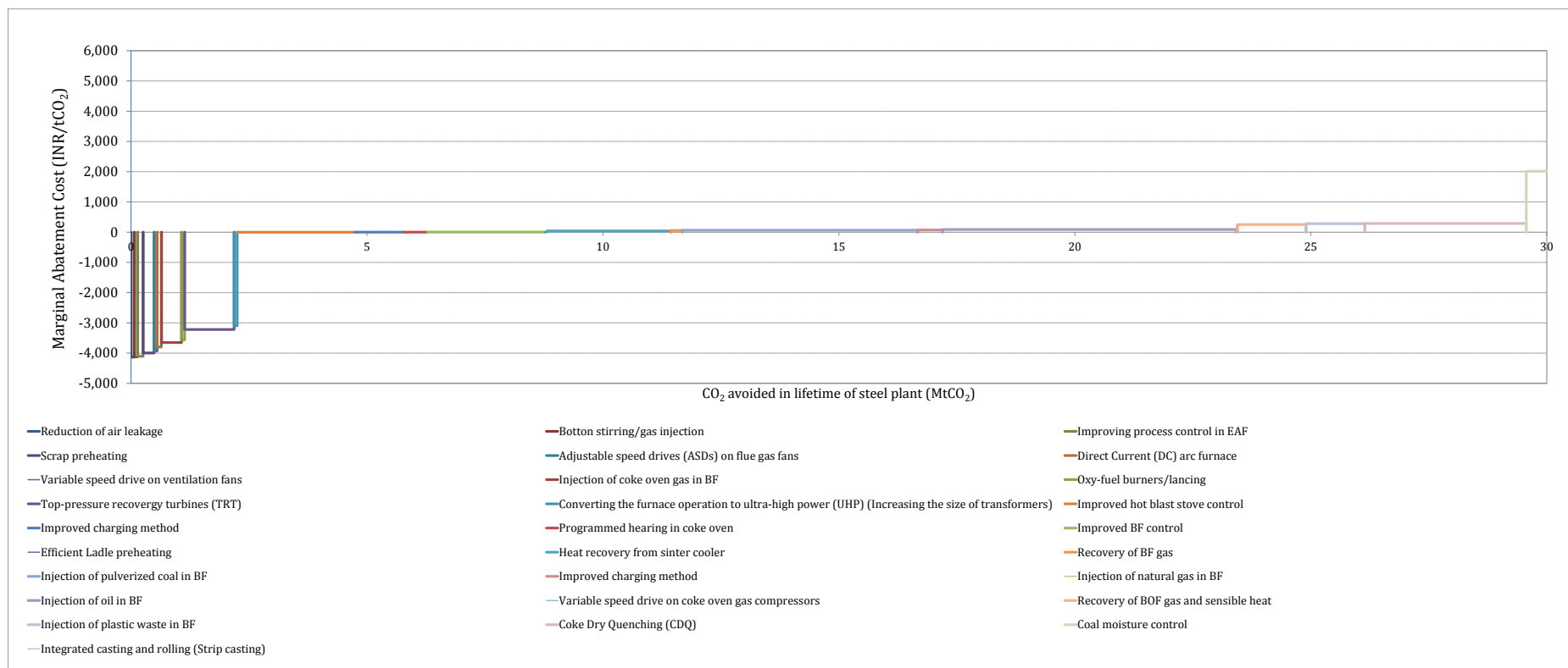
Figure 80: MAC curve for EE options in Iron and Steel Industry
