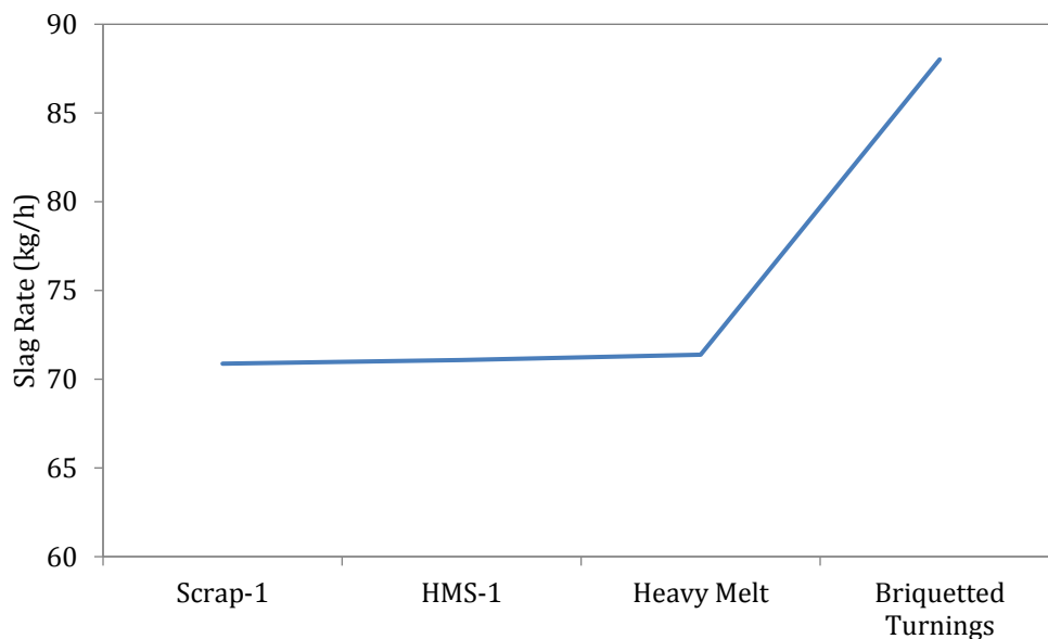
Figure 38: Slag rate vs. scrap type
