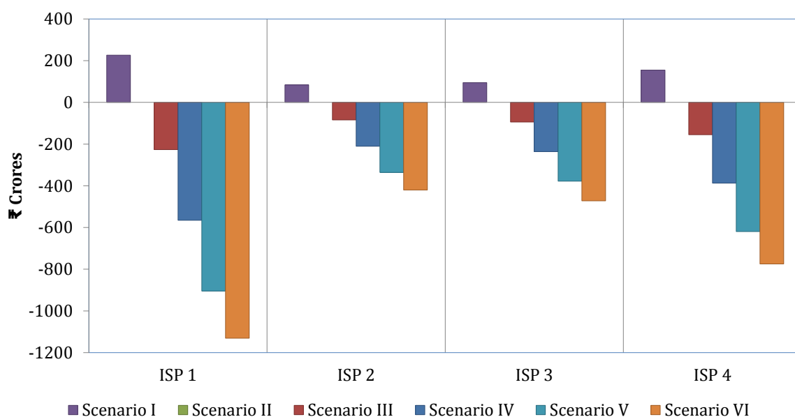
Figure 84: Savings beyond target under High Cost Scenario for Sample ISP plants
