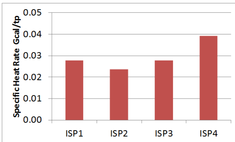
Figure 58: Specific Heat Rate in Sinter Plant for Sample ISP Plants
