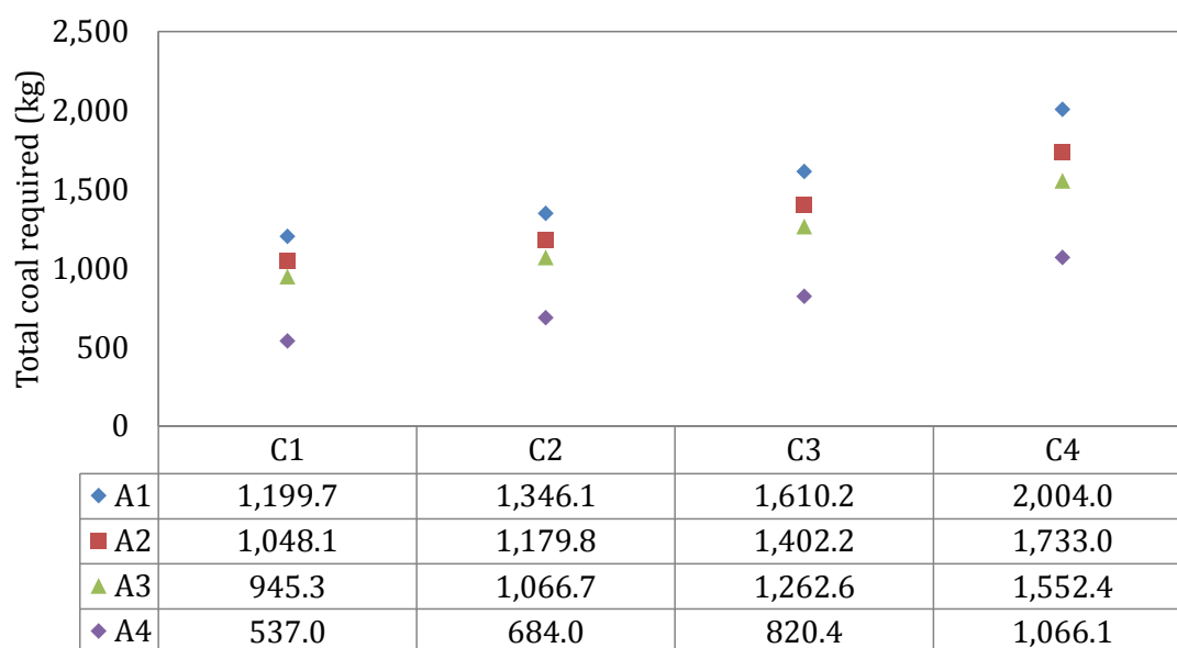
Figure 33: Coal required for different alternatives for iron ore 2
