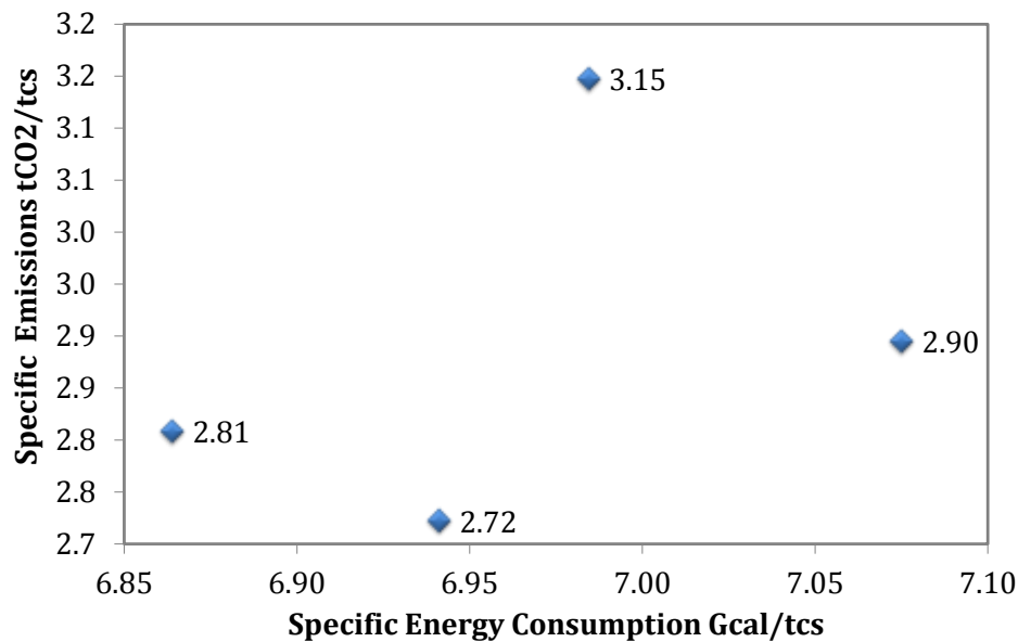
Figure 49: Comparisons of ISP Energy and Emission for Sample ISP Plants
