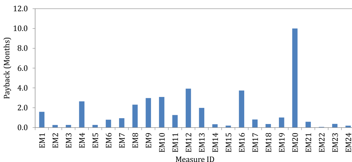
Figure 77; Payback period of different EE measures
