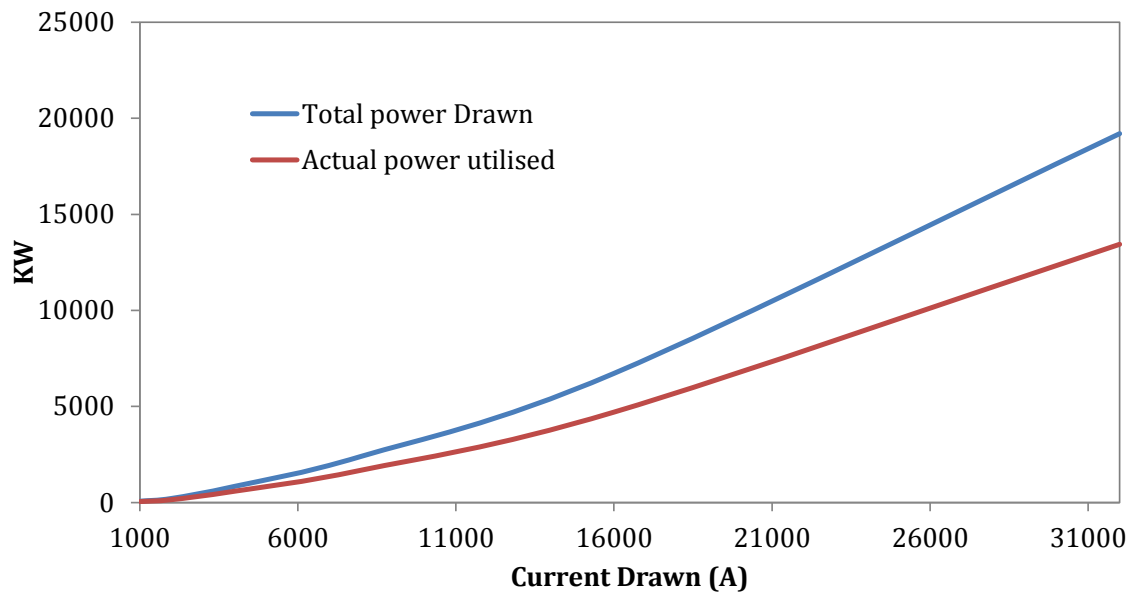
Figure 45: Actual power utilized vs. Power Drawn
