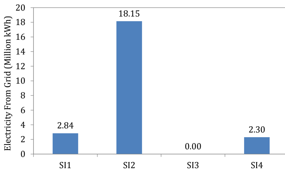
Figure 68: Purchased electricity from grid for sample SI plants
