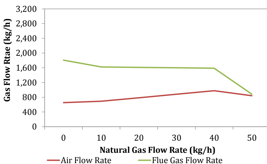
Figure 24: Hot Stove Performance with Mixed Fuel Injection
