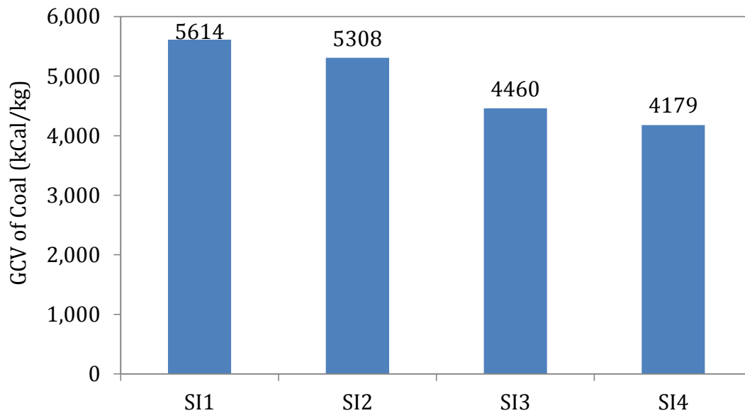
Figure 71: Gross Calorific Value (GCV) of different coals for sample SI plants
