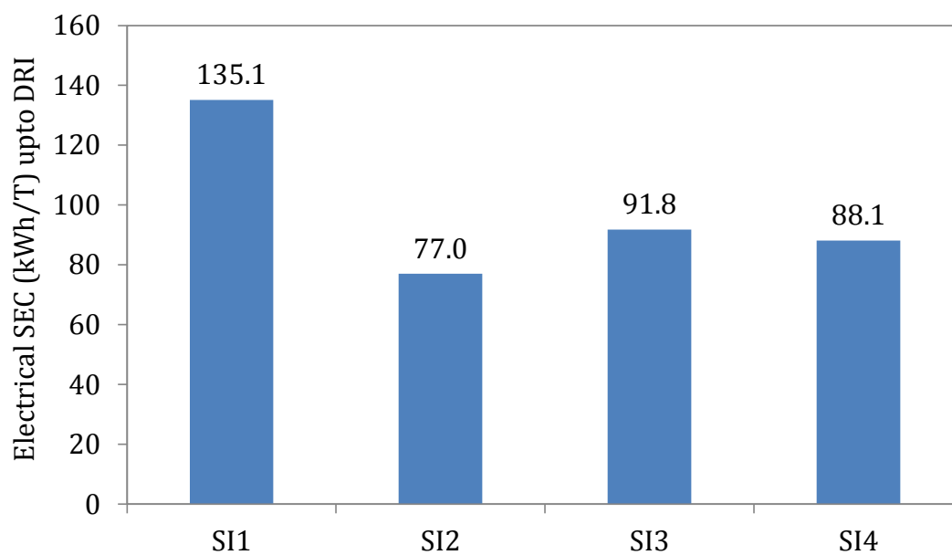
Figure 73: Electrical SEC of sponge iron making for sample SI plants
