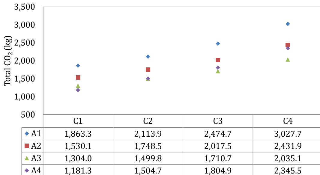
Figure 32: Total CO 2 emissions for different coals and for iron ore 1
