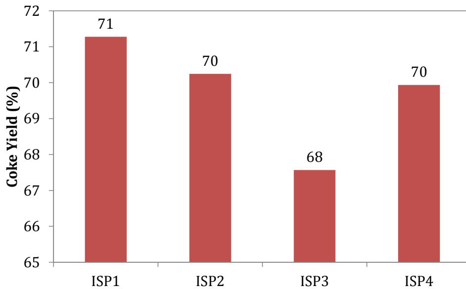
Figure 53: Coke Oven Yield for Sample ISP Plants
