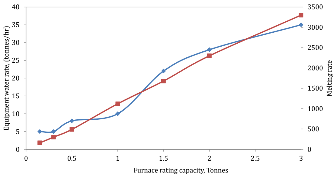
Figure 42: Furnace performance on melting rate and water consumption rate with increasing capacity of furnace
