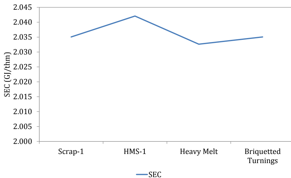
Figure 40: SEC of different scrap types
