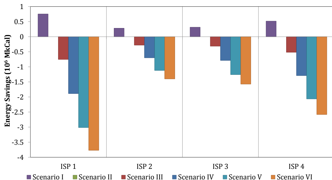
Figure 86. Energy saved beyond target for different Scenarios for Sample ISP plants
