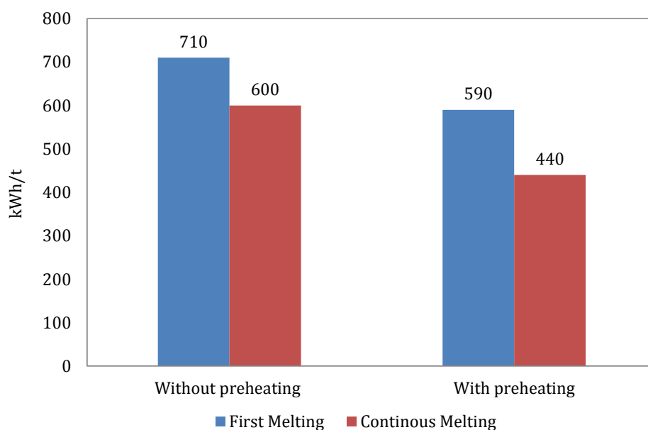
Figure 46: Comparison of equipment with and without preheating
