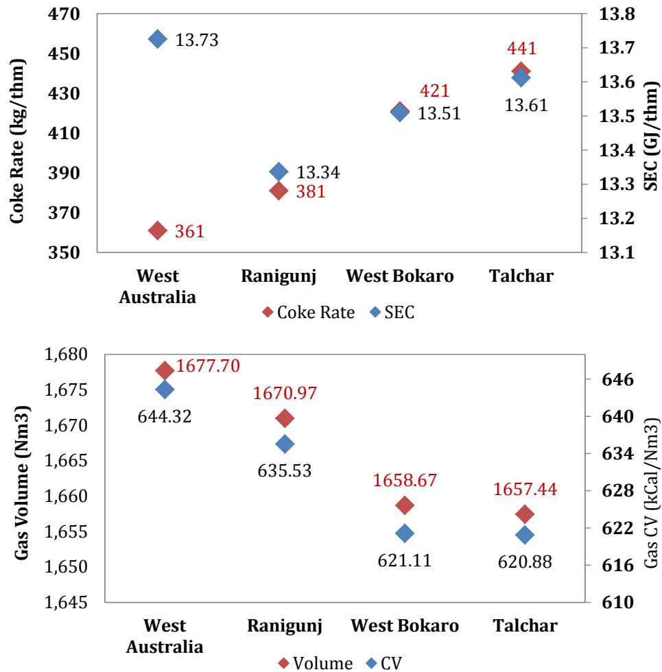
Figure 18: Parametric analysis on coal type and its effect on SEC
