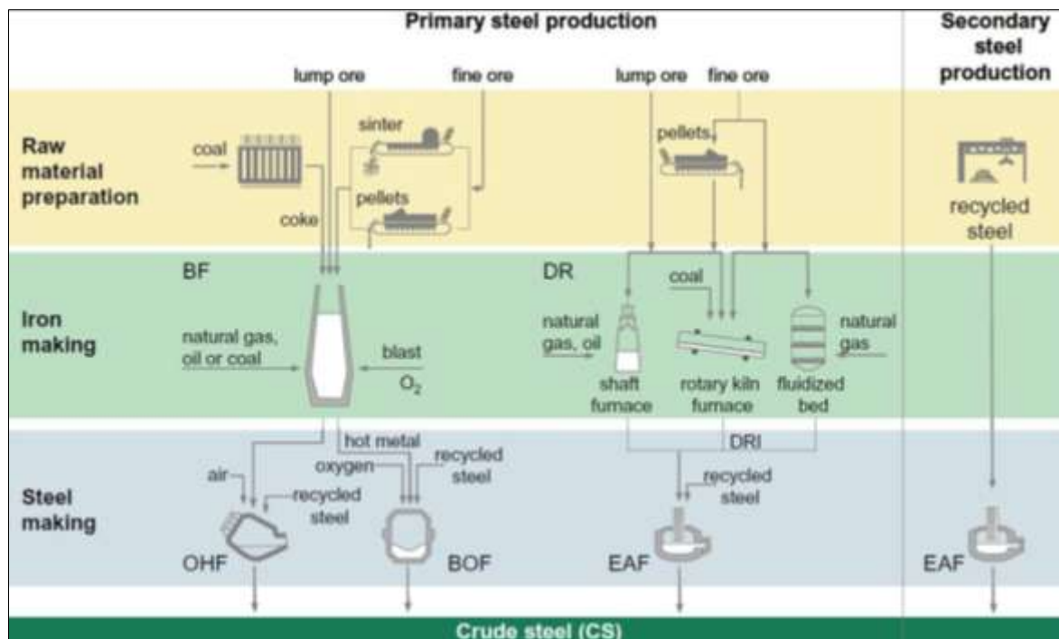
Figure 11 Iron and Steel Production Process routes (17)
