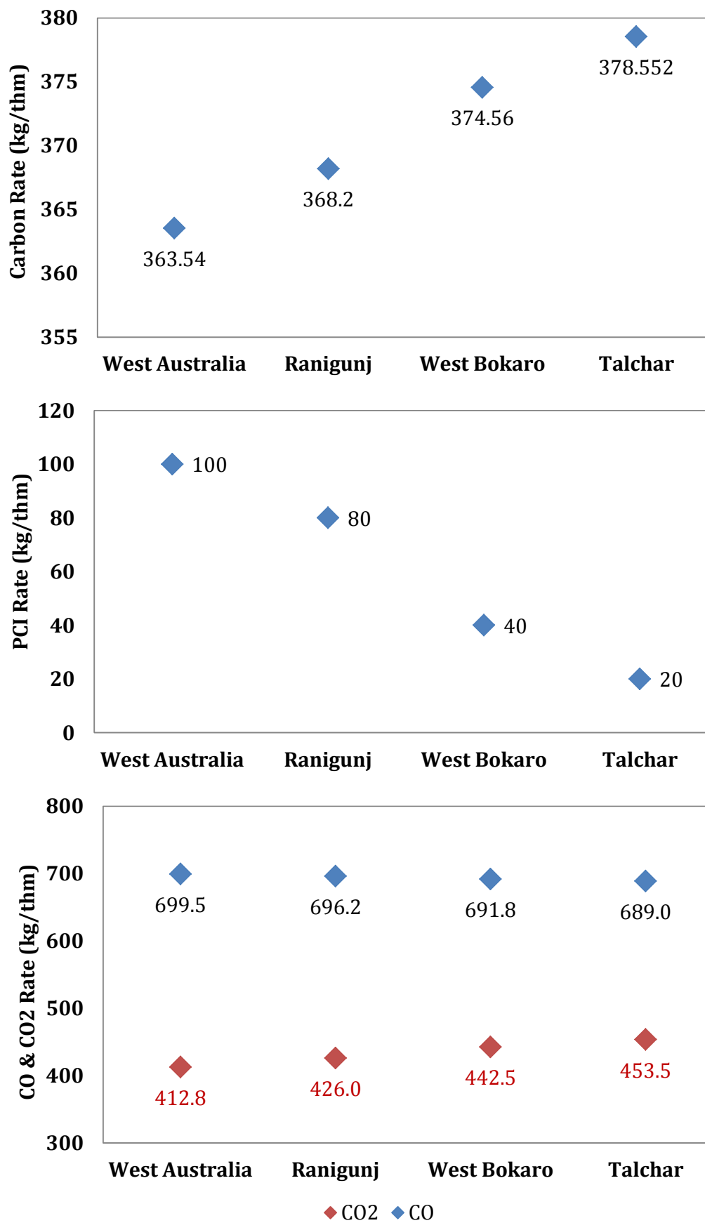
Figure 19: BF Performance with Coal Type
