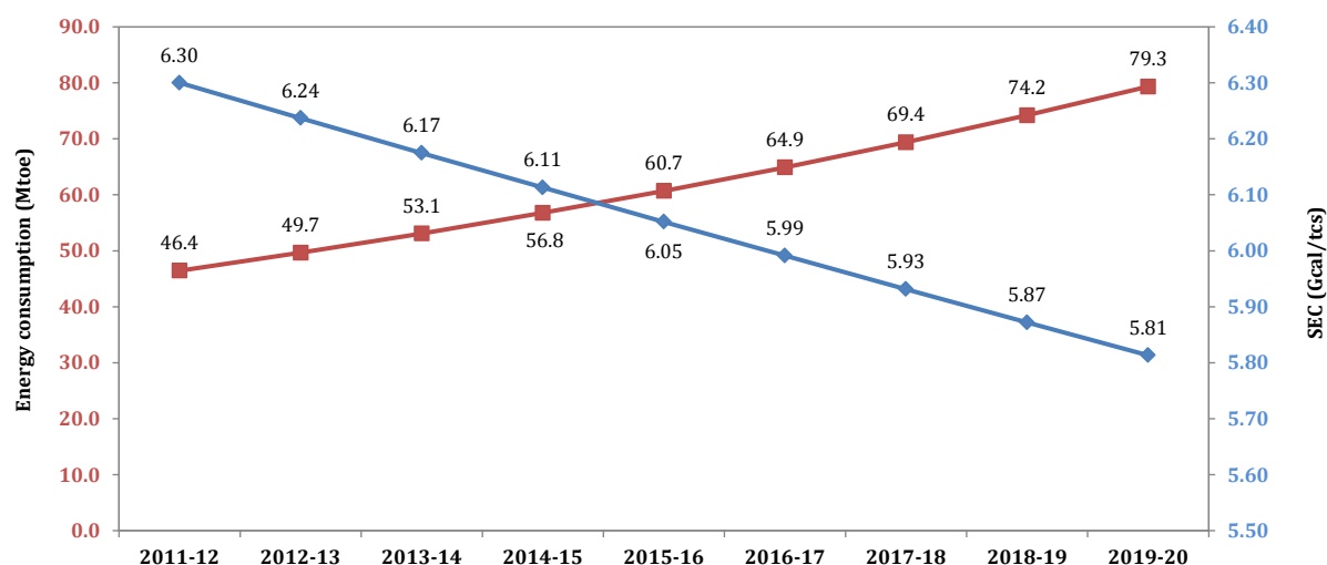
Figure 7: Projected Energy Consumption and Energy Intensity
