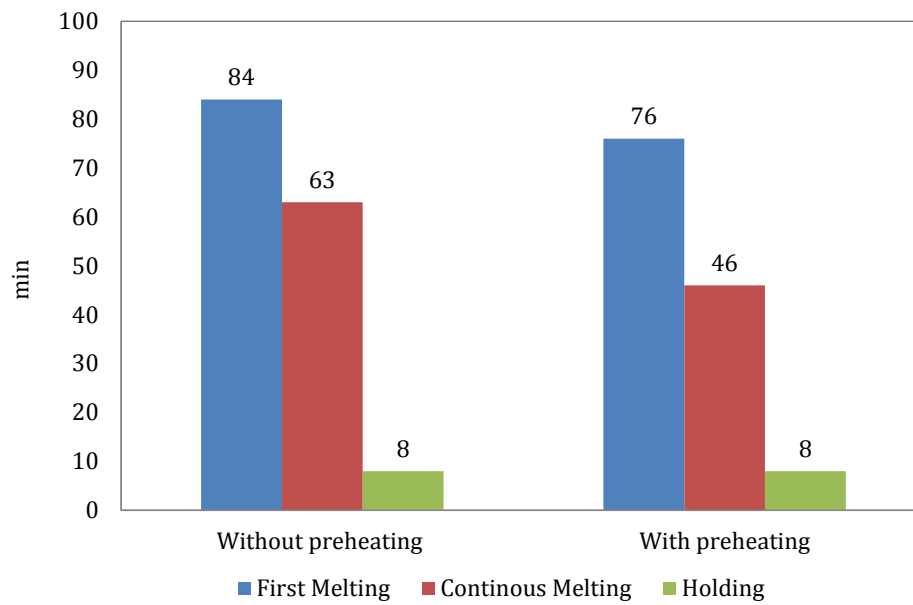
Figure 47: Review of melting time for equipment with and without preheating
