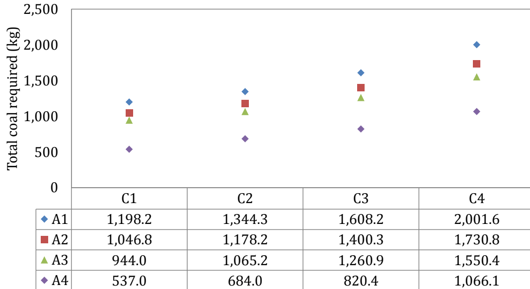
Figure 31: Coal required for different alternatives for iron ore 1
