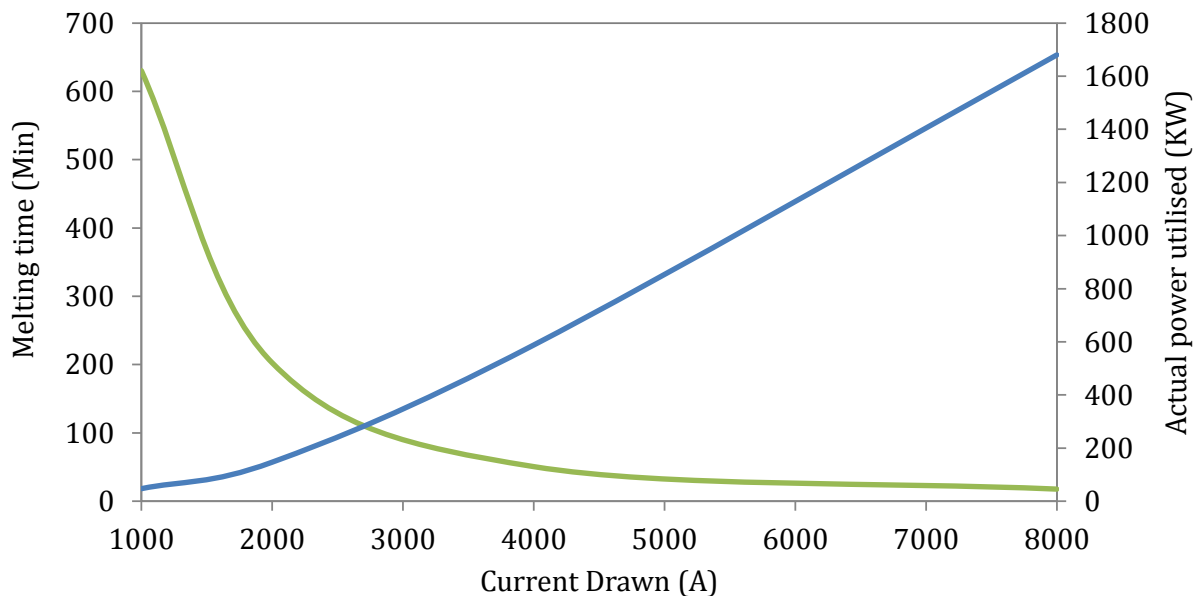
Figure 43: Performance of the furnace with respect to melting time and power utilized with increasing current drawn from the transformer
