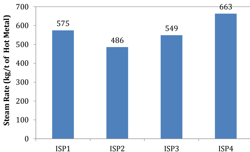
Figure 62: Steam Consumption Rate in Blast Furnace for Sample ISP Plants
