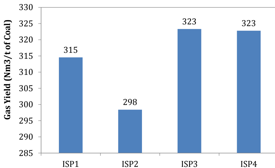
Figure 52: Coke Oven Gas Yield (At actual CV) for Sample ISP Plants
