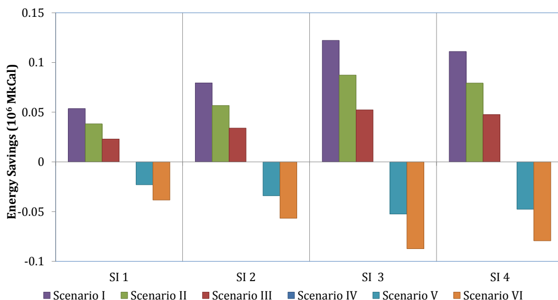
Figure 91: Energy saved at BL Production for different Scenarios for sample sponge iron plants
