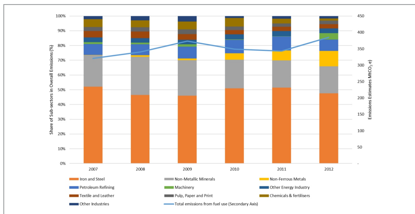
Figure 11: Sectoral Emissions of Fuel Use for the Period 2007-2012
