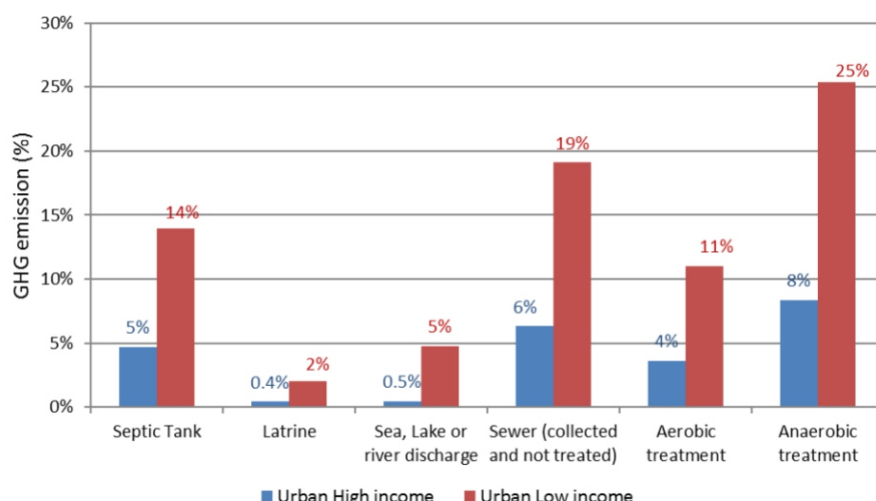
Figure 26: GHG Emission by Type of Domestic Wastewater Discharge/Treatment System for Urban-High Income and Urban-Low Income Groups in India (2012)
