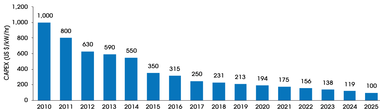
Graph 2: Past and projected trends in cost of lithium-ion batteries
