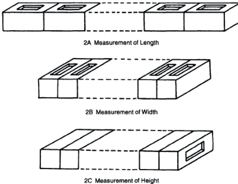
FIG. 2 MEASUREMENT OF TOLERANCES OF COMMON BUILDING BRICKS
