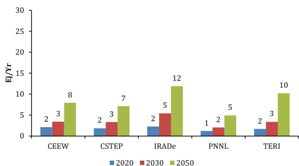
Figure 4: Transport-sector energy consumption: freight
