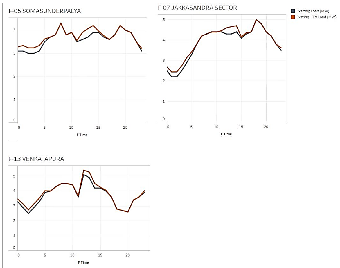
Figure 13: Feeder load comparison
