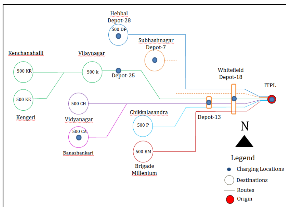
Figure 3: Feasible ITPL routes with charging locations (Vaira Buses)
