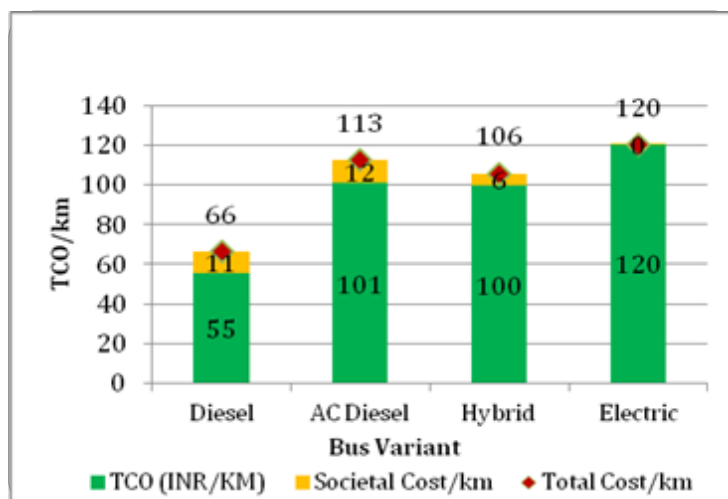
Figure 21: Pragmatic Case Scenario
