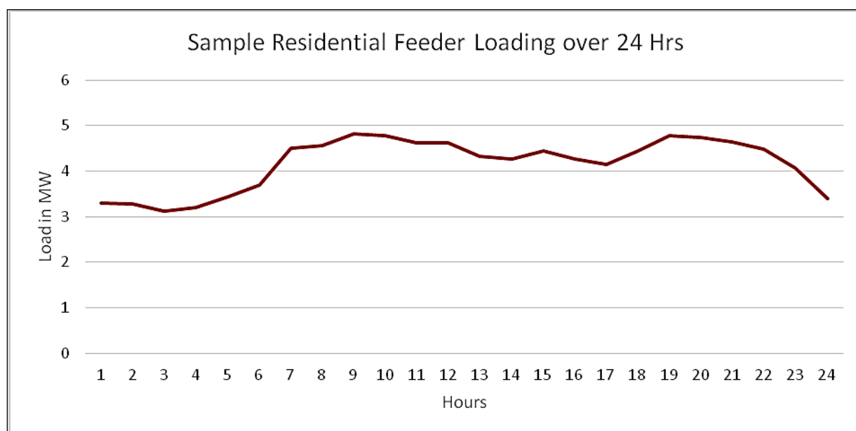
Figure 36: Electrical loading of a residential feeder (24 hours)
