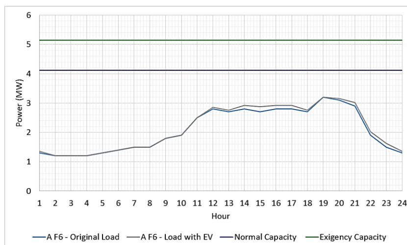
Figure 26: Electrical load on feeder F-6 (at Depot 7) caused by e-buses
