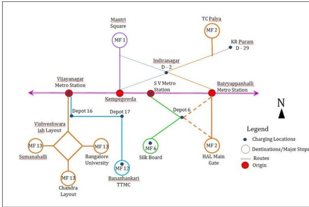
Figure 4: Feasible Metro-feeder routes with charging locations
