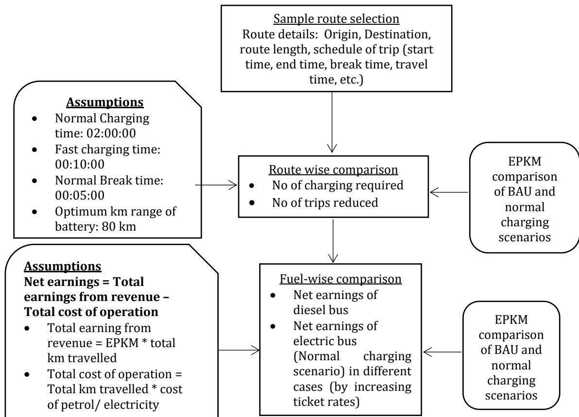
Figure 14: General methodology for the viability study of short-range battery buses
