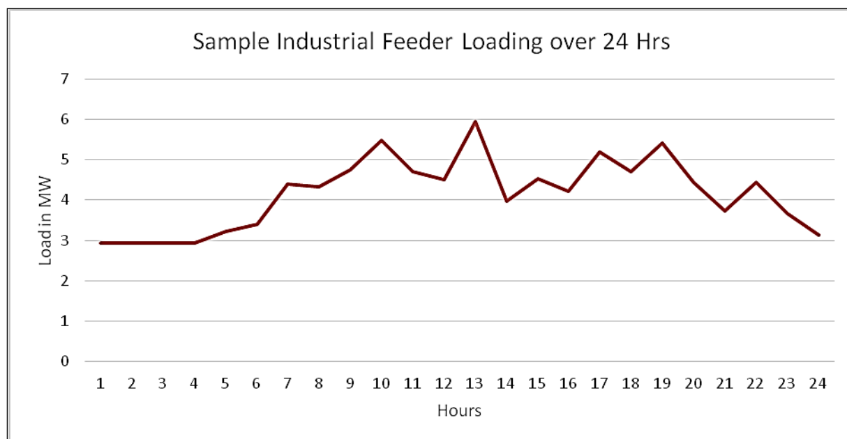
Figure 35: Electrical loading of an industrial feeder (24 hours)
