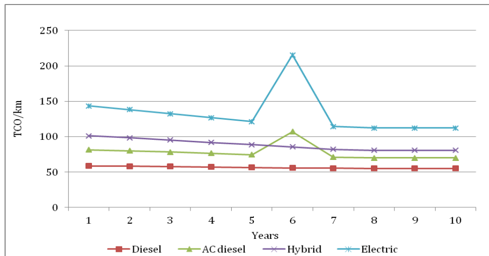
Figure 18: Year-wise TCO/km for the lifetime of a bus
