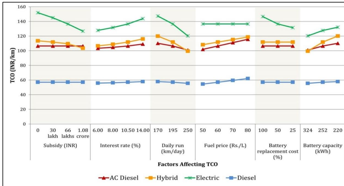
Figure 19: Summary of effects of individual parameters on TCO
