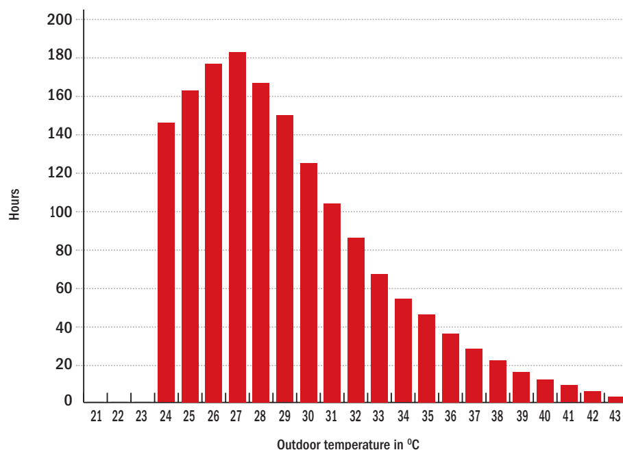
Graph 13: Reference outdoor temperature bin distribution for Indian SEER
