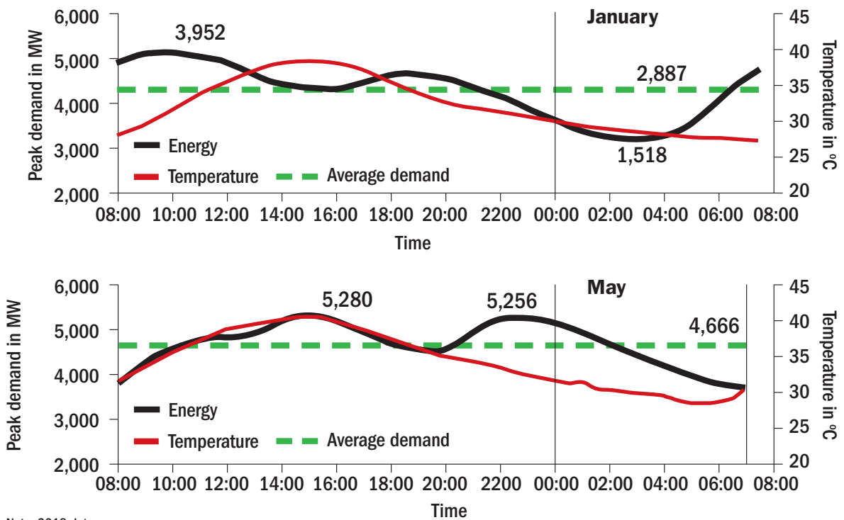
Graph: Typical electricity demand pattern in January and May
