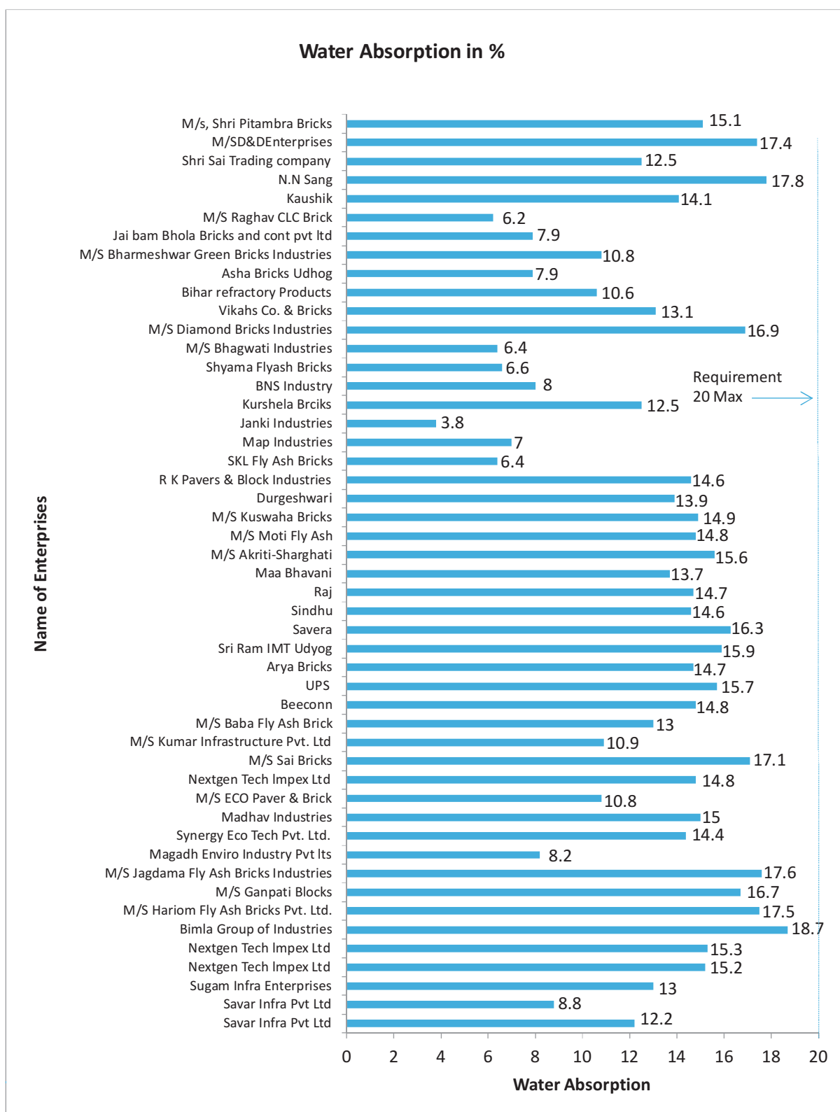
Figure 19: Graph on quality testing results – Water Absorption
