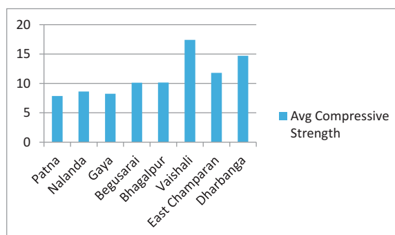
Figure 18: Average compressive strength in selected districts of Bihar
