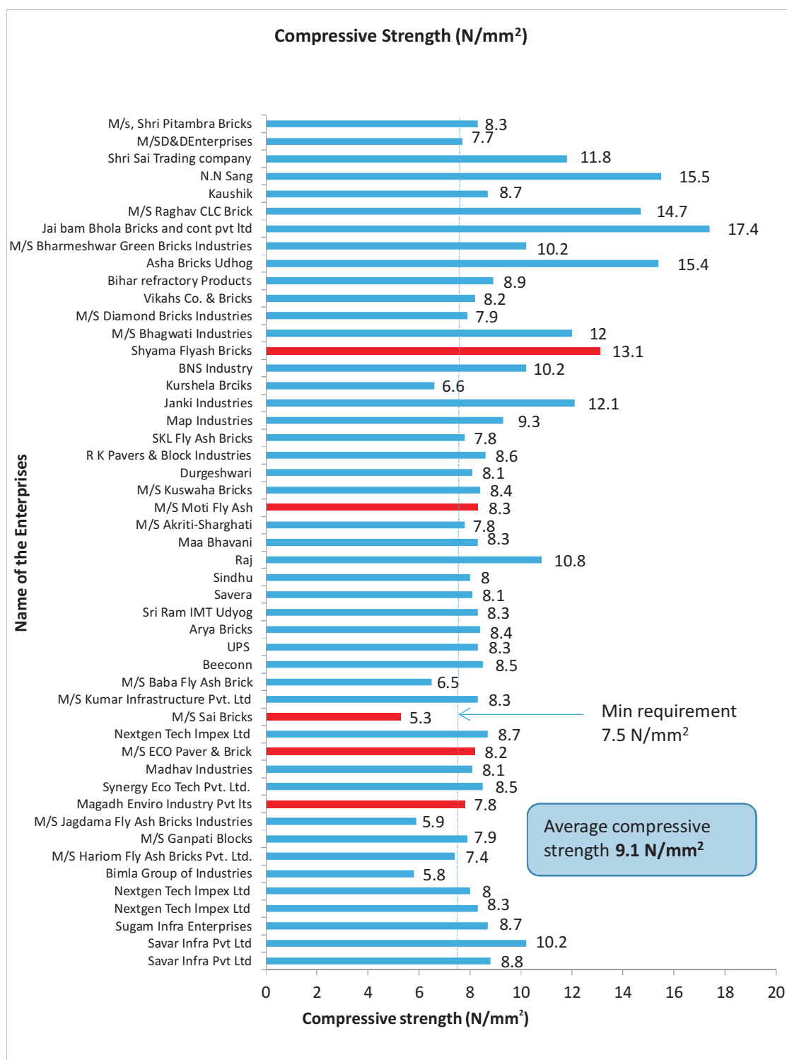
Figure 20: Graph on quality testing results – Compressive strength
