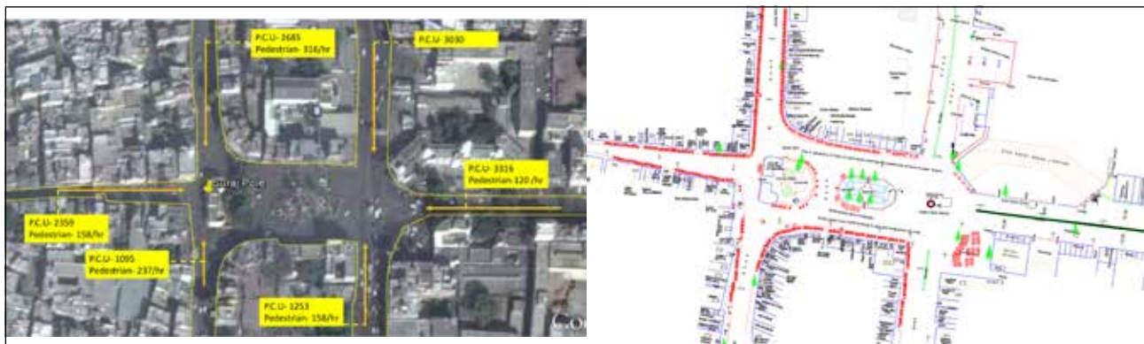
Figure 2.: Traffic Volume Count(Left) and Activity Mapping (Right) at Suraj Pole
