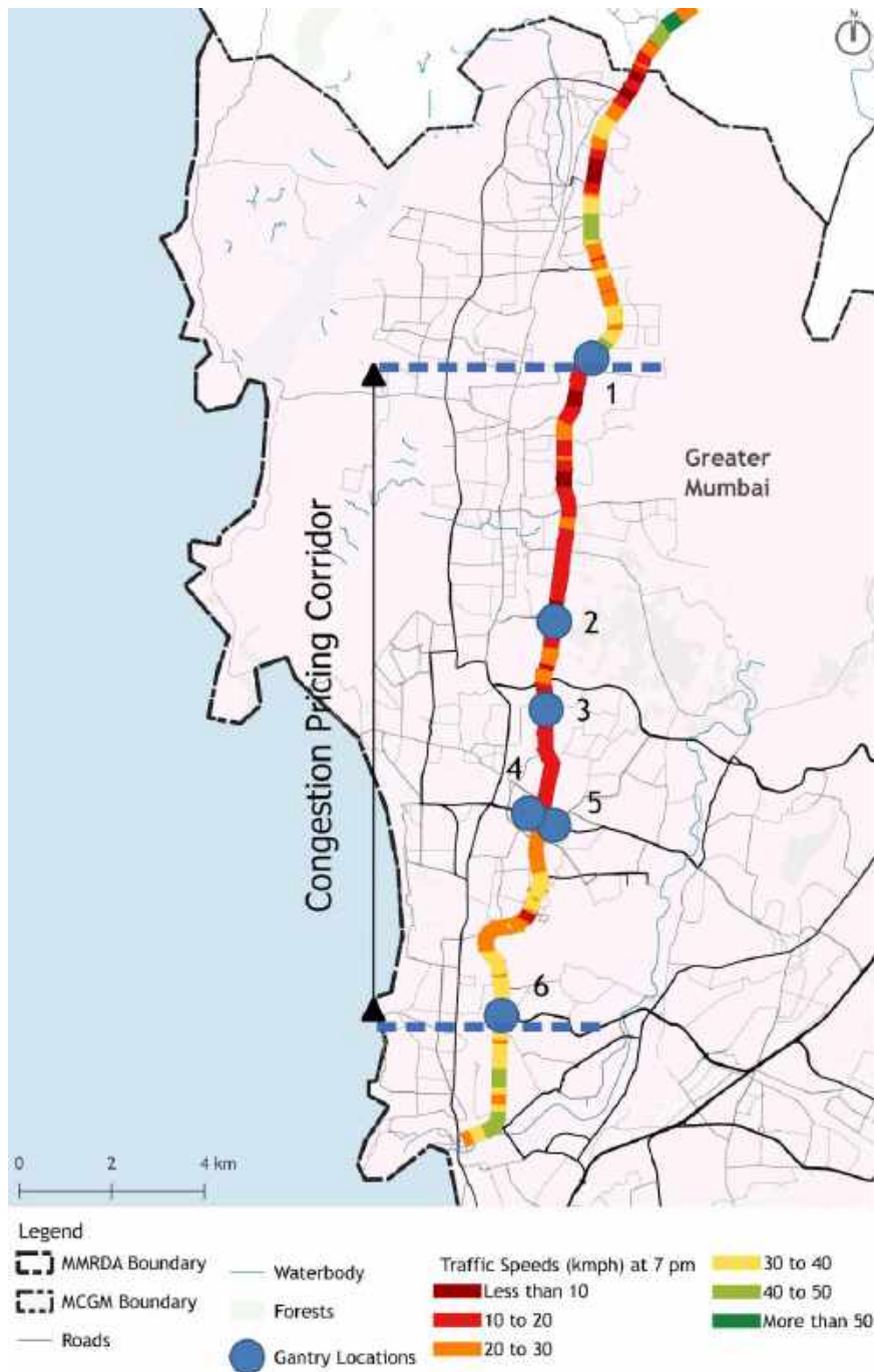
Figure 30 Location of congestion pricing gantries on WEH
