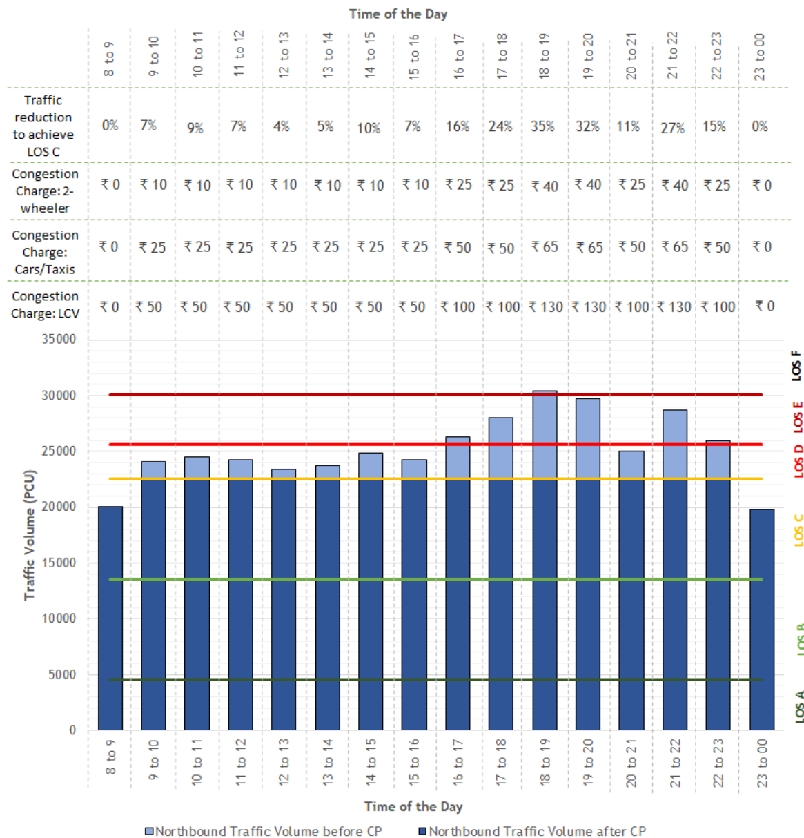
Figure 28 Traffic volume reduction and deterrent charges required for northbound traffic in Island City
