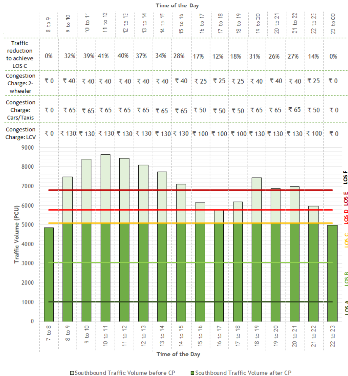
Figure 32 Traffic volume reduction and deterrent charges required for southbound traffic on Western Express Highway (WEH) near Andheri
