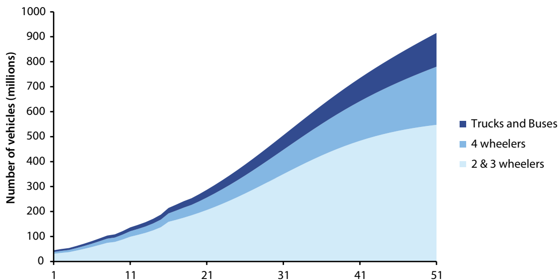
Figure 11: Projection of the stock of automobiles, 2000–50
