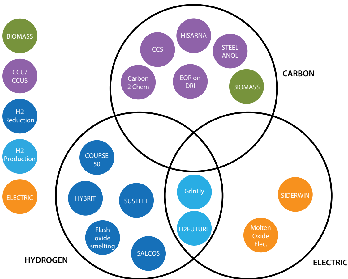
Figure 46: Overview of decarbonization technology projects for the iron and steel sector
