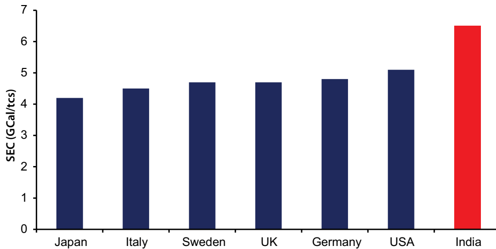
Figure 4: Average specific energy consumption of integrated steel plants by country
