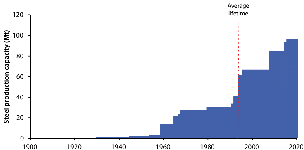
Figure 5: Production capacity of large steel plants by year of establishment
