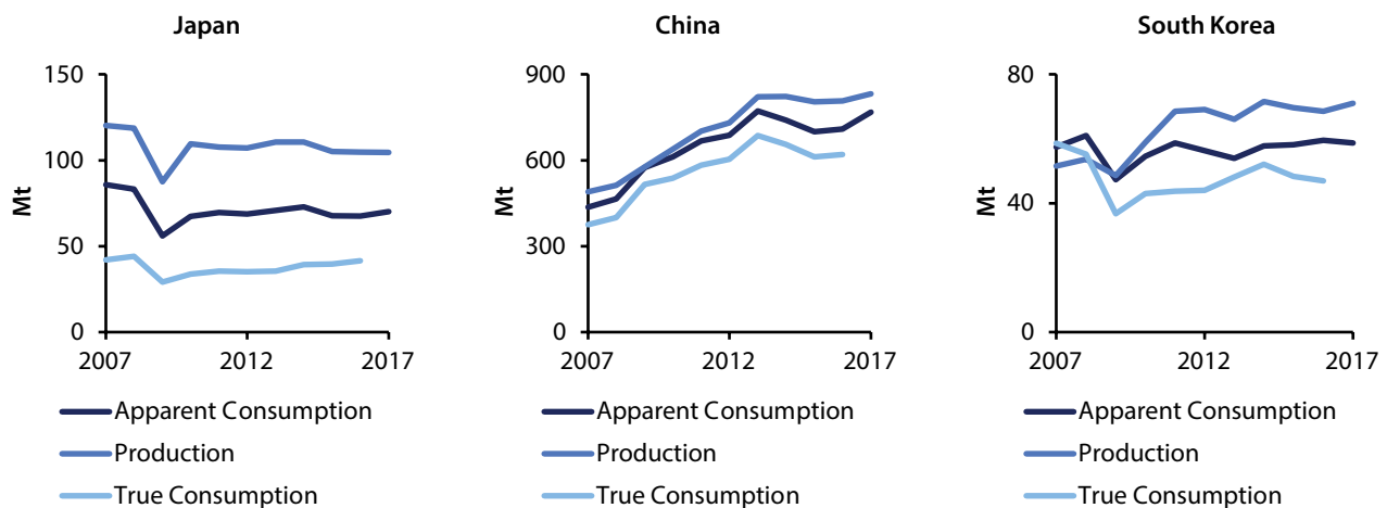
Figure 40: Production versus apparent consumption and true steel consumption: China, Japan and South Korea (2007–17)
