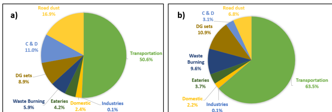
Figure 3-42: Sectoral contribution of a) NO x and b) SO 2 emissions over the air-shed area
