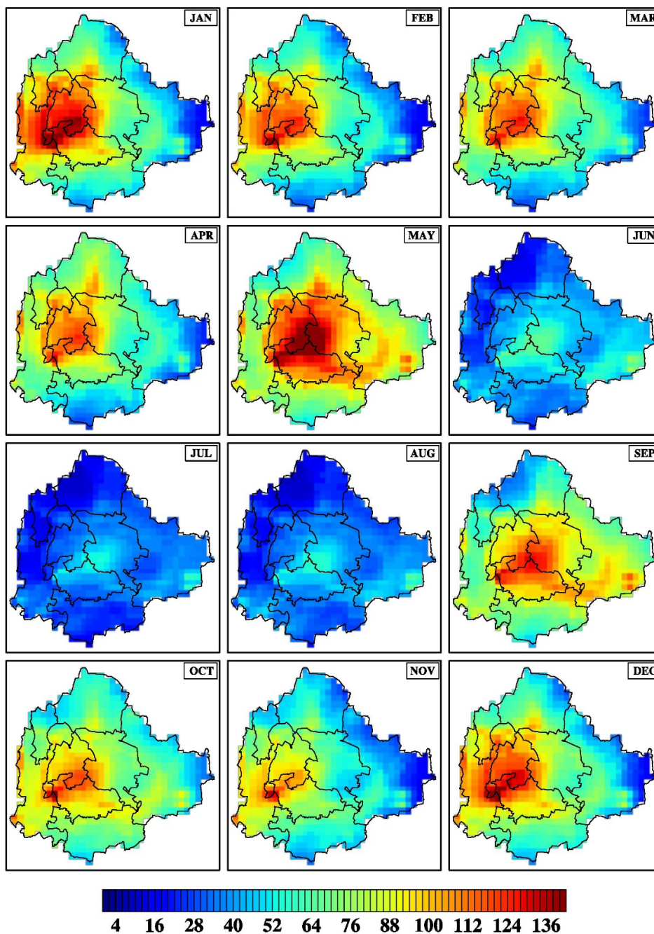
Figure 5-18: Monthly average values of WRF-CAMx-model-simulated PM 10 concentration (µg/m 3 ) during 2024 under high emission reduction scenario over Bengaluru
