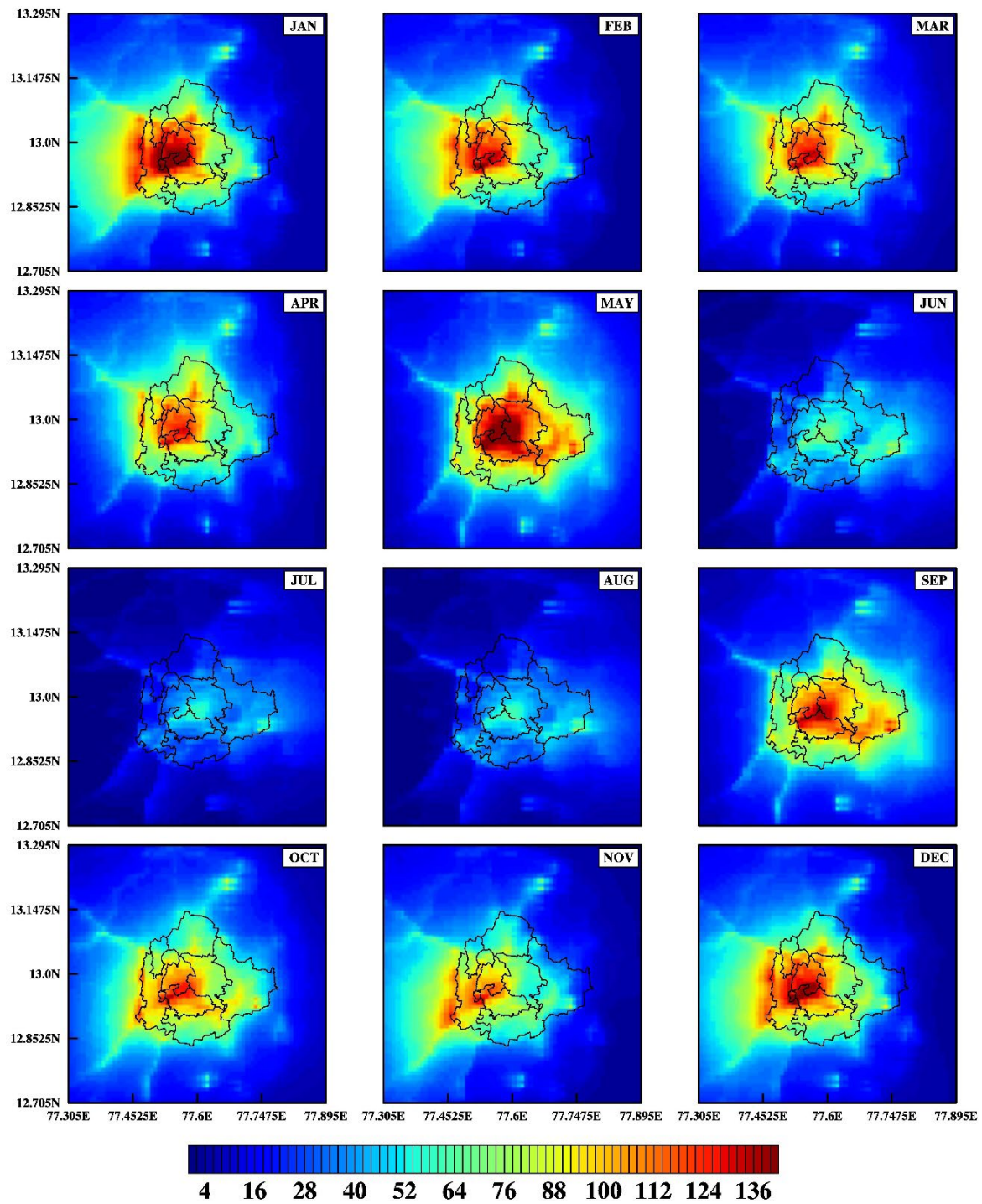
Figure 4-6: Monthly average values of simulated PM_{10} concentration ( \mu g/m^3 ) - 2019
