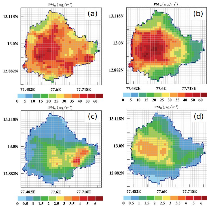
Figure 4-10: PM_{10} concentration ( \mu g/m^3 ) for a) dust, b) transportation, c) DG sets, & d) eateries
