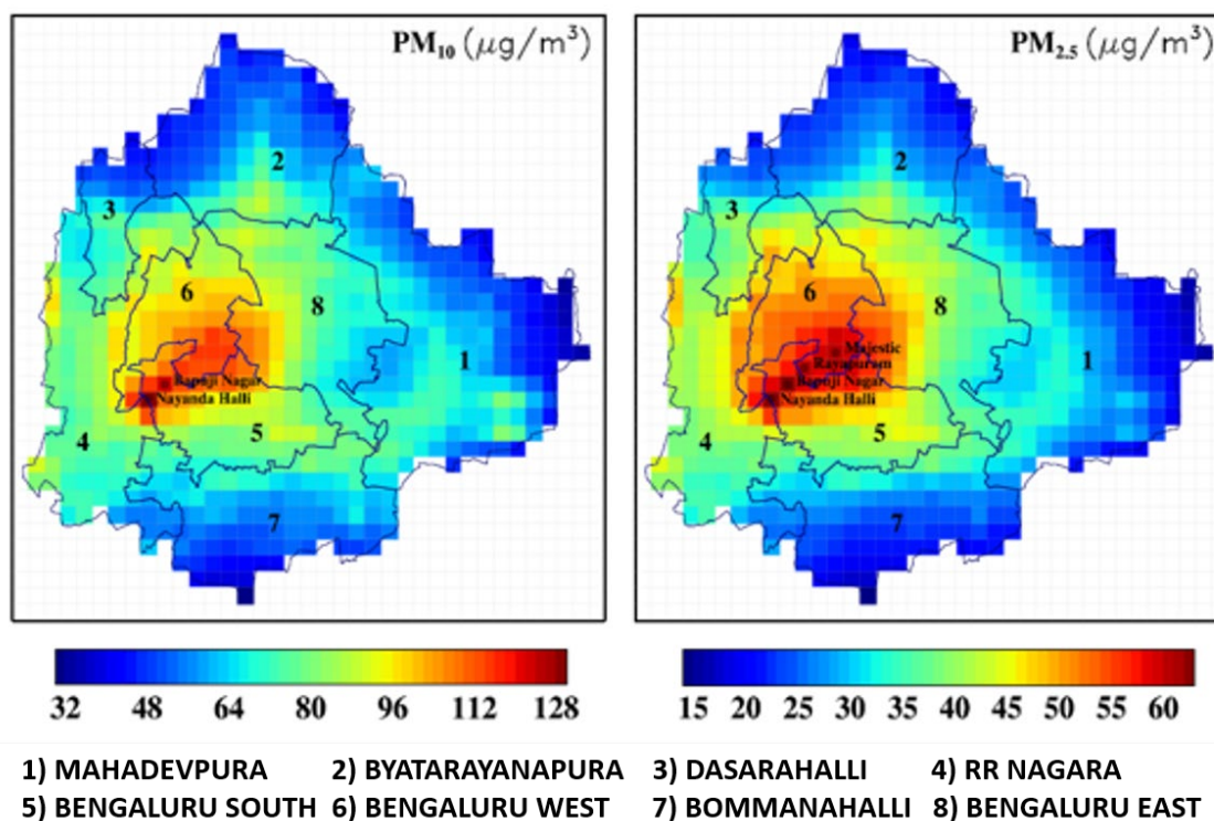
Figure 4-5: Mean annual average concentration values of simulated PM_{10} and PM_{2.5} ( \mu g/m^3 ) - 2019
