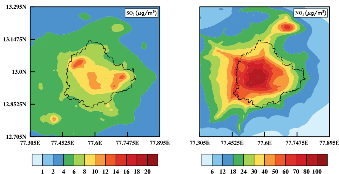
Figure 4-8: Annual average concentration of simulated \text{SO}_2 and \text{NO}_2 ( \mu\text{g}/\text{m}^3 ) - 2019
