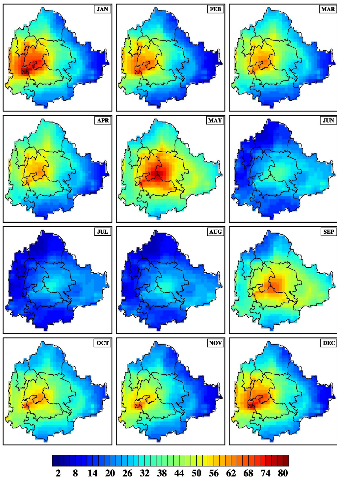
Figure 5-13: Monthly average values of WRF-CAMx-model-simulated PM 2.5 concentration (µg/m³) during 2024 under high emission reduction scenario over Bengaluru
