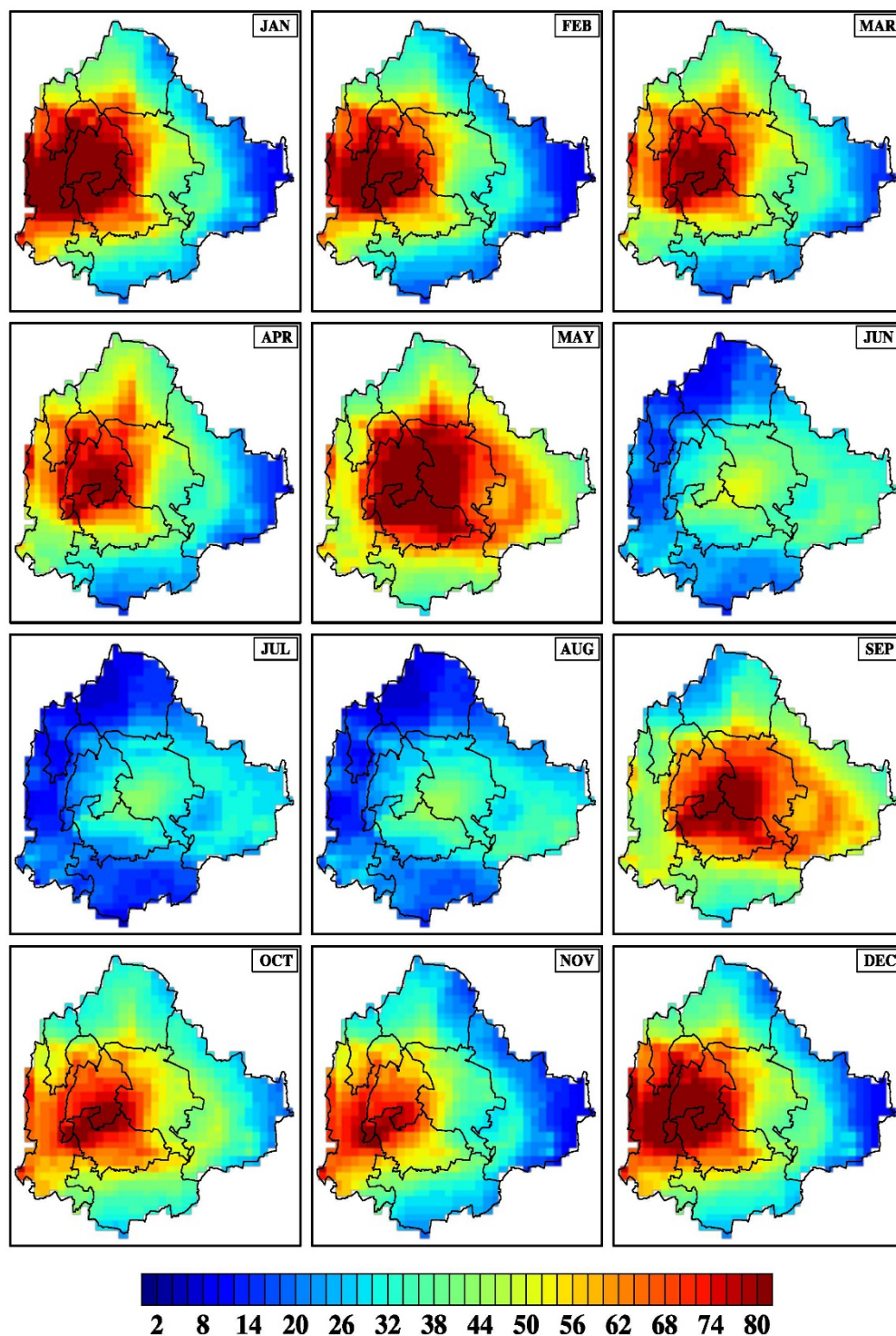
Figure 5-8: Mean monthly average concentration values of simulated PM 2.5 concentration (µg/m 3 ) during 2024 under BAU scenario
