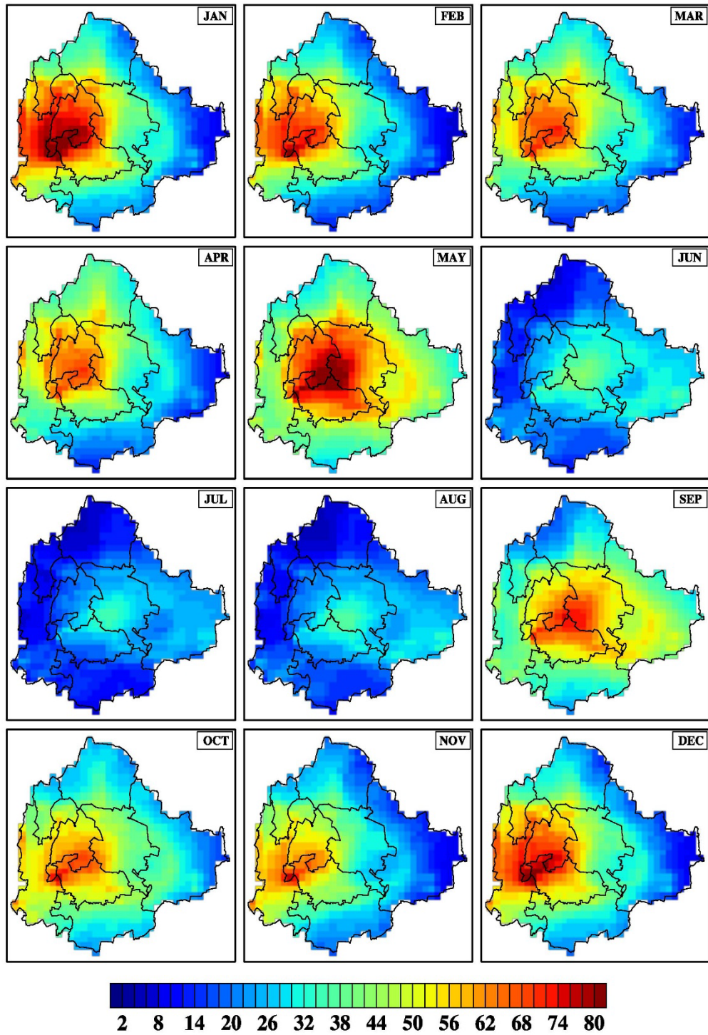
Figure 5-7: Monthly average concentration values of simulated PM 2.5 concentration (µg/m³) during 2020 under BAU scenario
