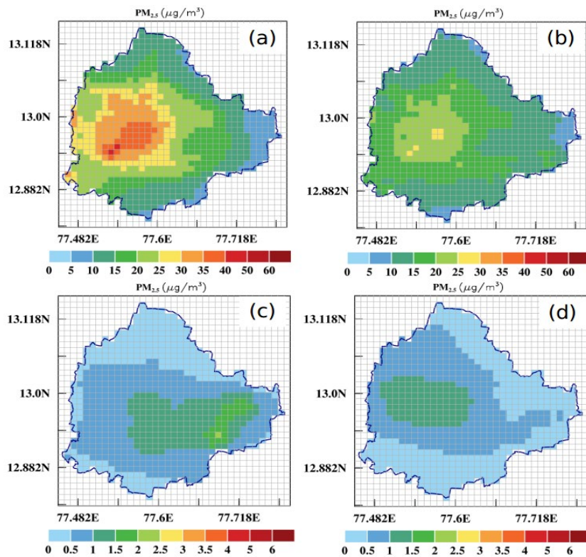
Figure 4-11: PM_{2.5} concentration ( \mu g/m^3 ) for a) dust, b) transportation, c) DG sets, & d) eateries
