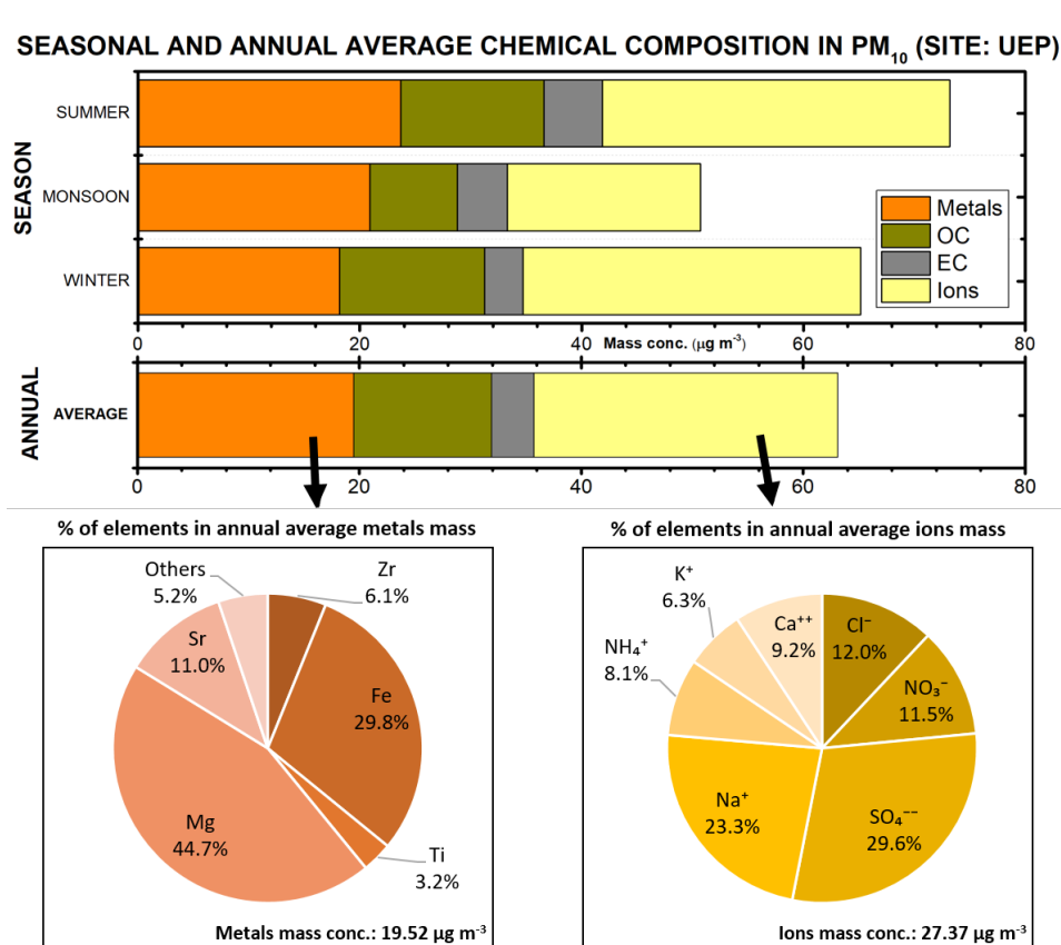
Figure 37: Seasonal and annual average chemical composition in \text{PM}_{10} . The pie charts indicate the % of elements in annual average of metals and ions mass.
