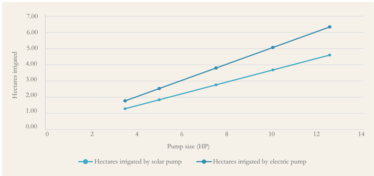
Figure 11: Solar pumps are constrained by available radiation during seasons of high water demand, so may be able to support fewer farmers year-round
