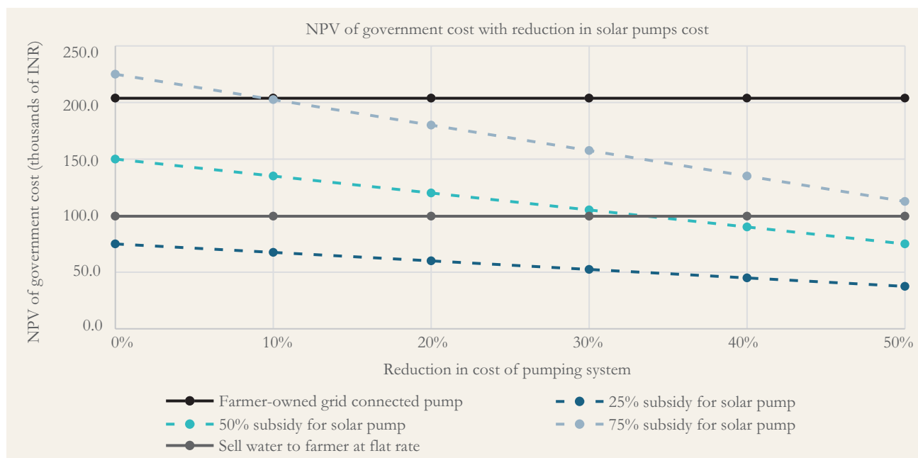
Figure 9: Under modest reductions in pump and panel prices, the government could provide generous subsidies for solar pumps at a lower cost than supporting electric pumps
