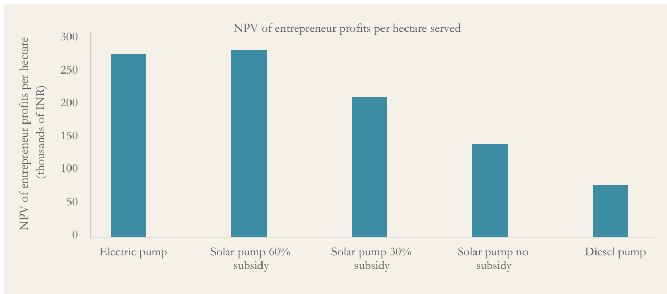
Figure 4: High utilisation under water-as-a-service model makes solar more attractive than diesel
