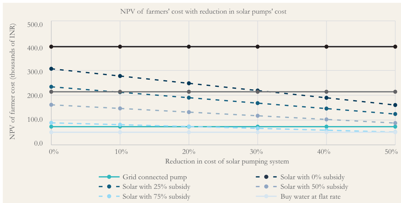
Figure 8: Decreasing pump and panel costs could change farmer's preference between solar and diesel pumps
