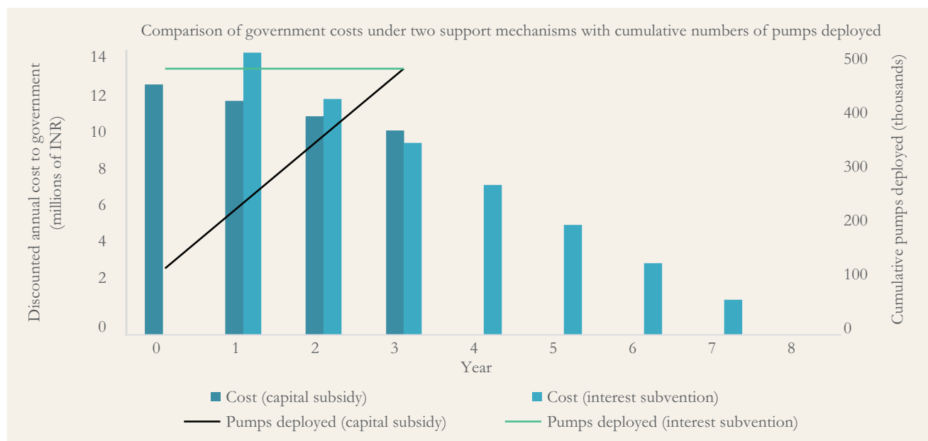
Figure 7: Government could increase the pace of solar pump deployment under interest subvention without incurring high upfront costs
