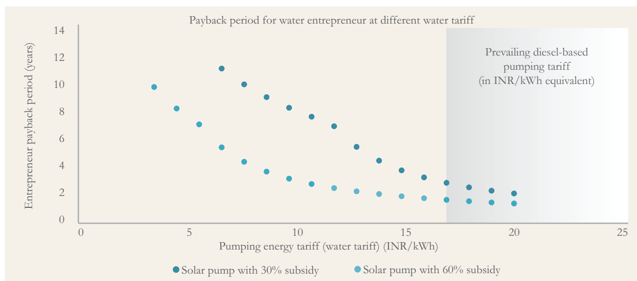
Figure 5: With 30 per cent capital subsidy, a solar entrepreneur could undercut tariff of a diesel pump operator and expect a payback period of under three years
