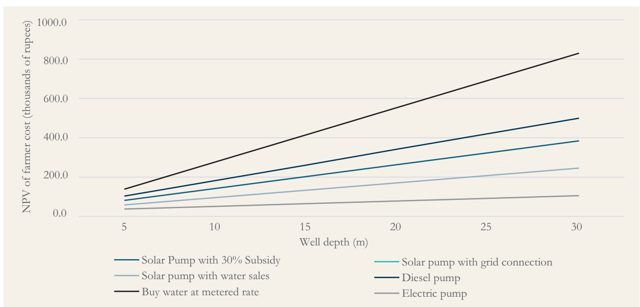
Figure 13: NPV of farmer cost to irrigate vs. well depth
