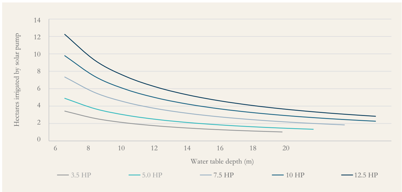
Figure 12: Pump flow rate is sensitive to well depth. Shallower wells and higher flow rates enable greater sharing of solar pumps
