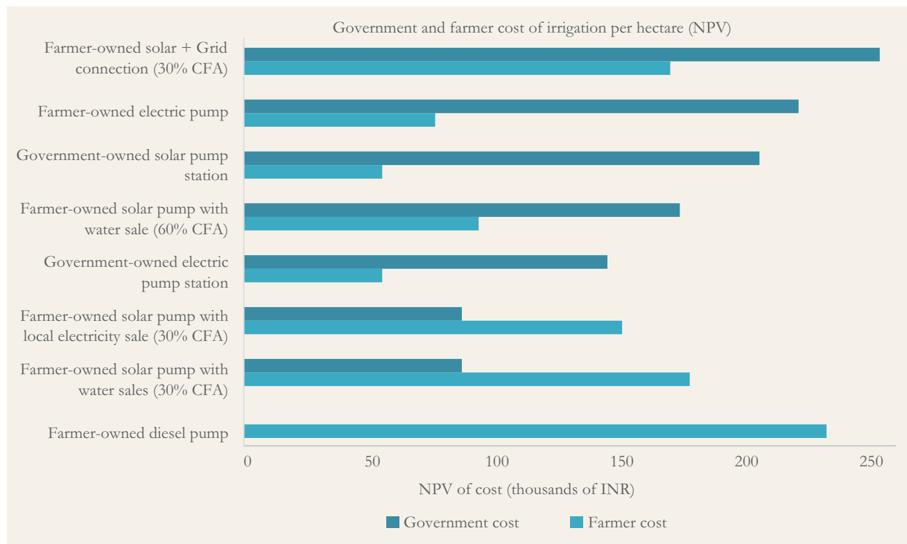
Figure 3: Comparing farmer and government per-hectare cost across pumping options
