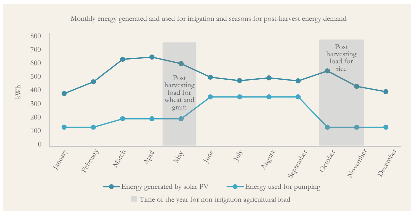
Figure 2: Surplus energy from solar pumps is well-suited for seasonal applications
