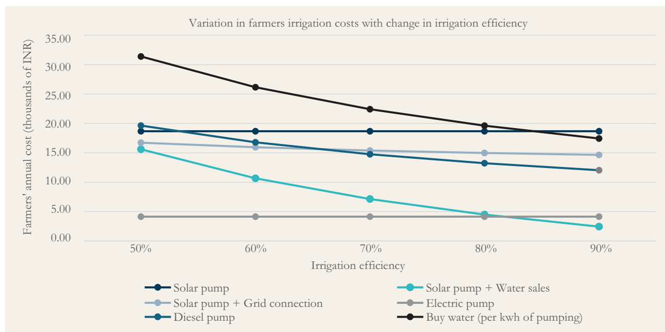
Figure 10: Farmers who sell water or electricity locally from solar pump can improve their economic outlook by improving irrigation efficiency
